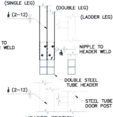
6 HEADER SECTION
