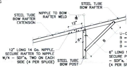
9 BOW/POST DETAIL
