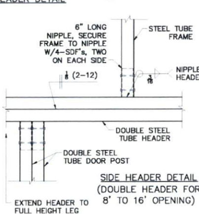
7 BOW / HEADER DETAIL
