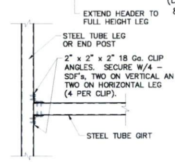
4 GIRT TO POST CONNECTION
