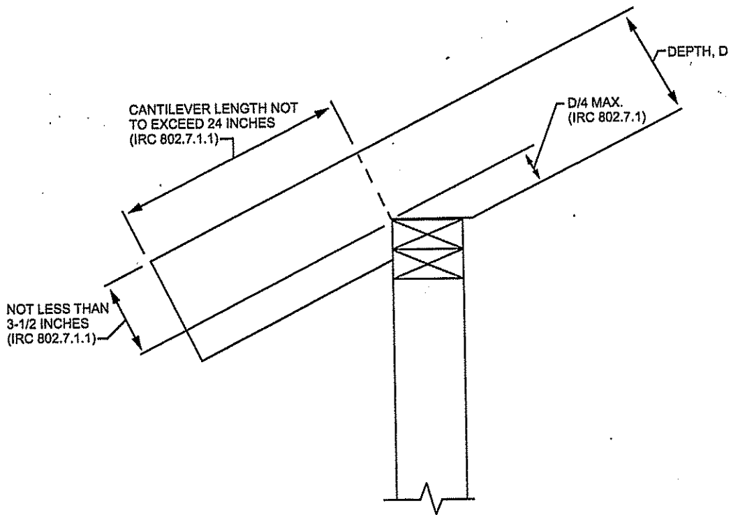
FIGURE R802.7.1.1
