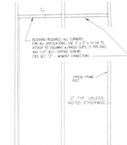
SECTION 3-3 (PARTIAL) NOT TO SCALE
