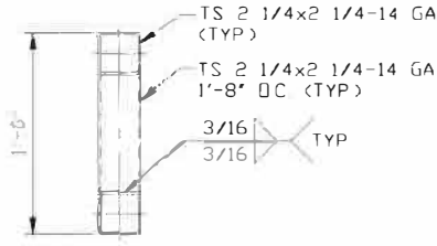
HEADER DETAIL FOR SIDE WALL DOOR OPENINGS 11'-0" < LENGTH ≤ 20'-0" SCALE: NTS
