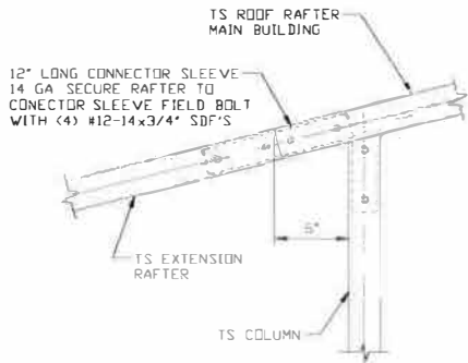
13 SIDE EXTENSION RAFTER/COLUMN DETAIL FOR SPAN \le 10'-0''
