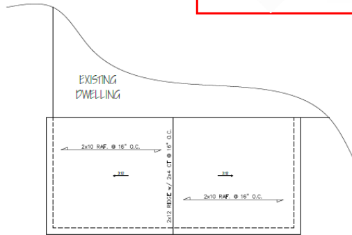
ROOF PLAN 1/4" = 1'-0"
