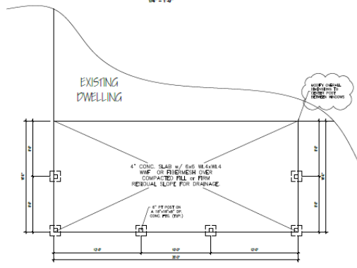
FOUNDATION PLAN 1/4" = 1'-0"
