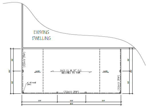
STRUCTURAL PLAN 1/4" = 1'-0"
