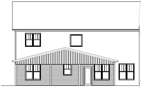
REAR ELEVATION 1/4" = 1'-0"
