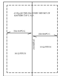
ROOF PLAN SCALE: 1/4" = 1'-0"
