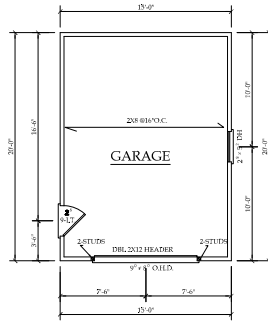
FLOOR PLAN SCALE: 1/4" = 1'-0"
