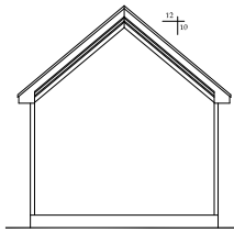
REAR ELEVATION SCALE: 1/4" = 1'-0"
