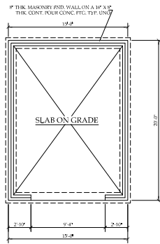
FOUNDATION PLAN SCALE: 1/4" = 1'-0"
