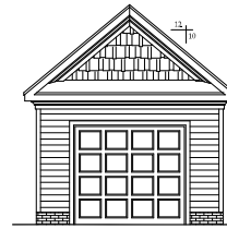
FRONT ELEVATION SCALE: 1/4" = 1'-0"
