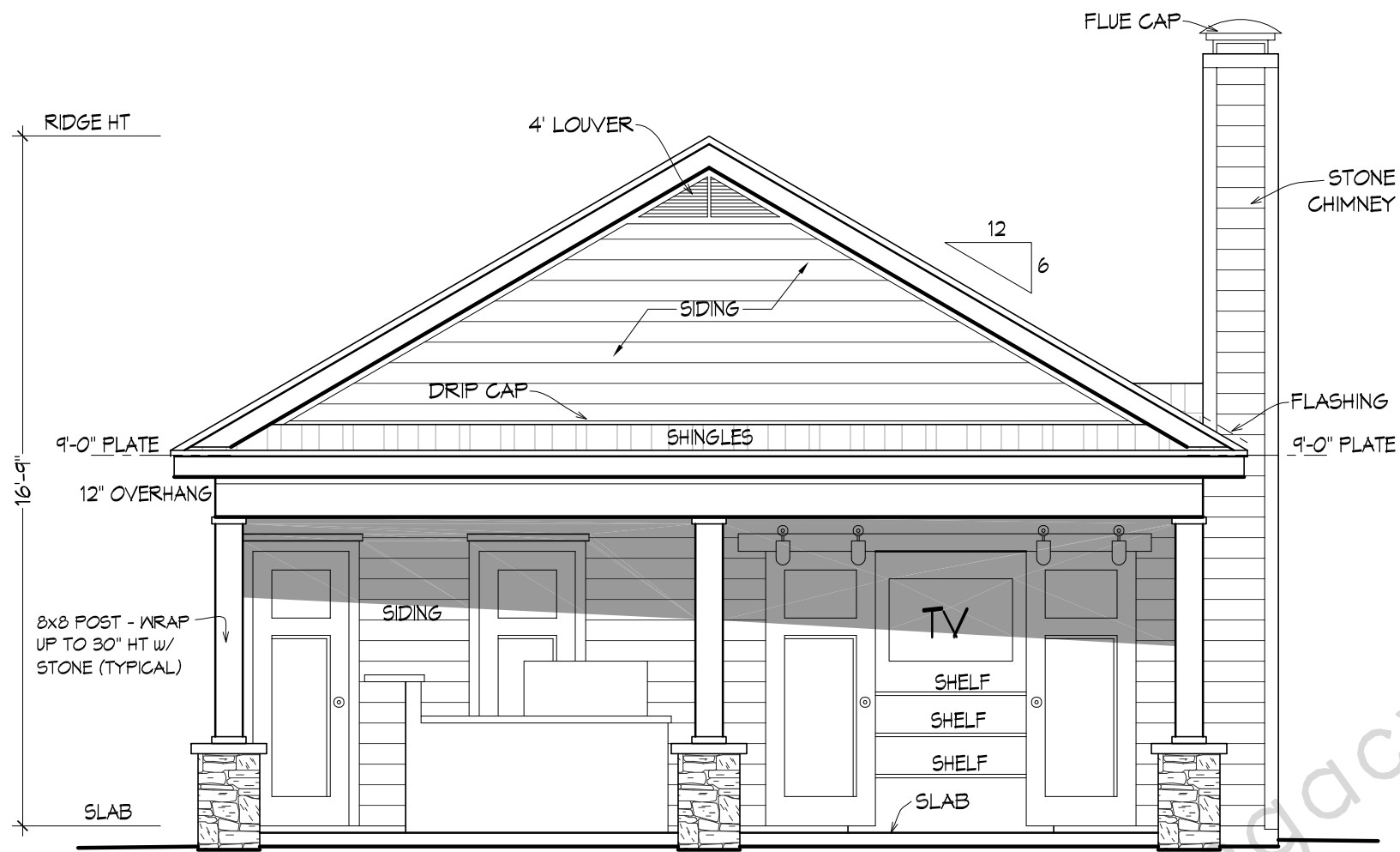
SCALE: 1/4" = 1'-0" FRONT ELEVATION
