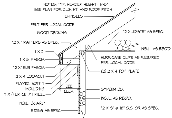
TYPICAL CORNICE DETAIL W/ SIDING NO SCALE
