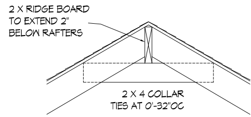
TYPICAL RIDGE BOARD / BRACING NO SCALE
