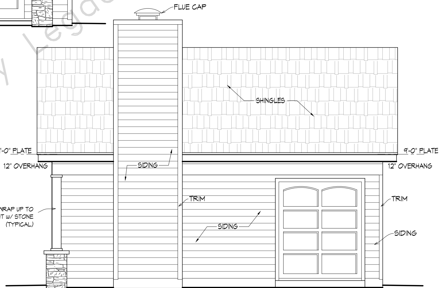
SCALE: 1/4" = 1'-0" RIGHT SIDE ELEVATION
