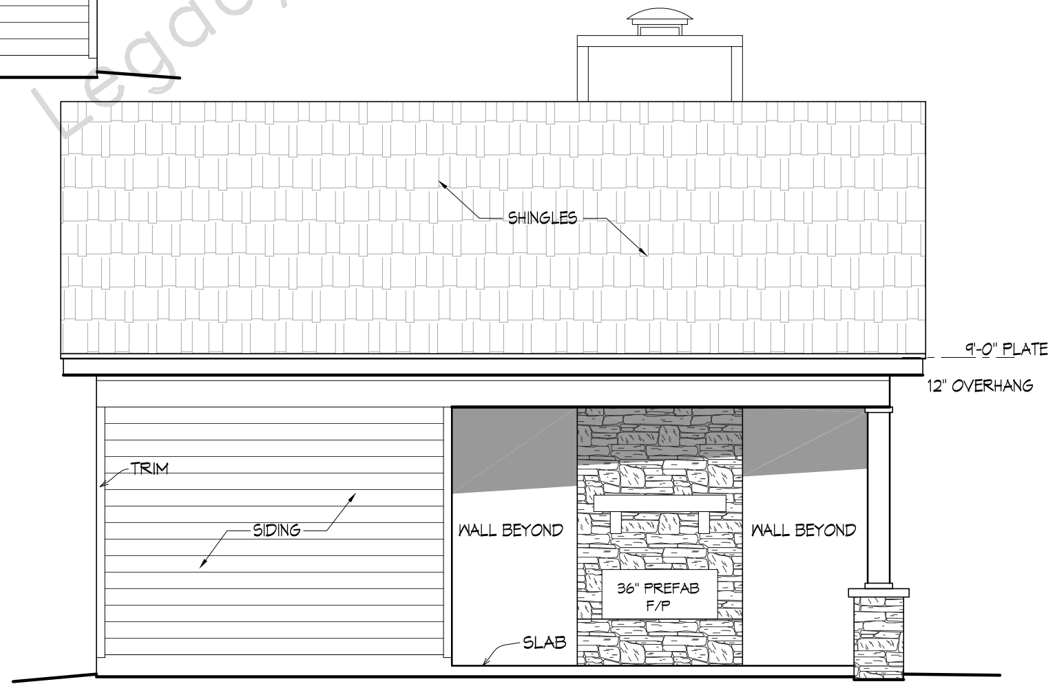
SCALE: 1/4" = 1'-0" LEFT SIDE ELEVATION
