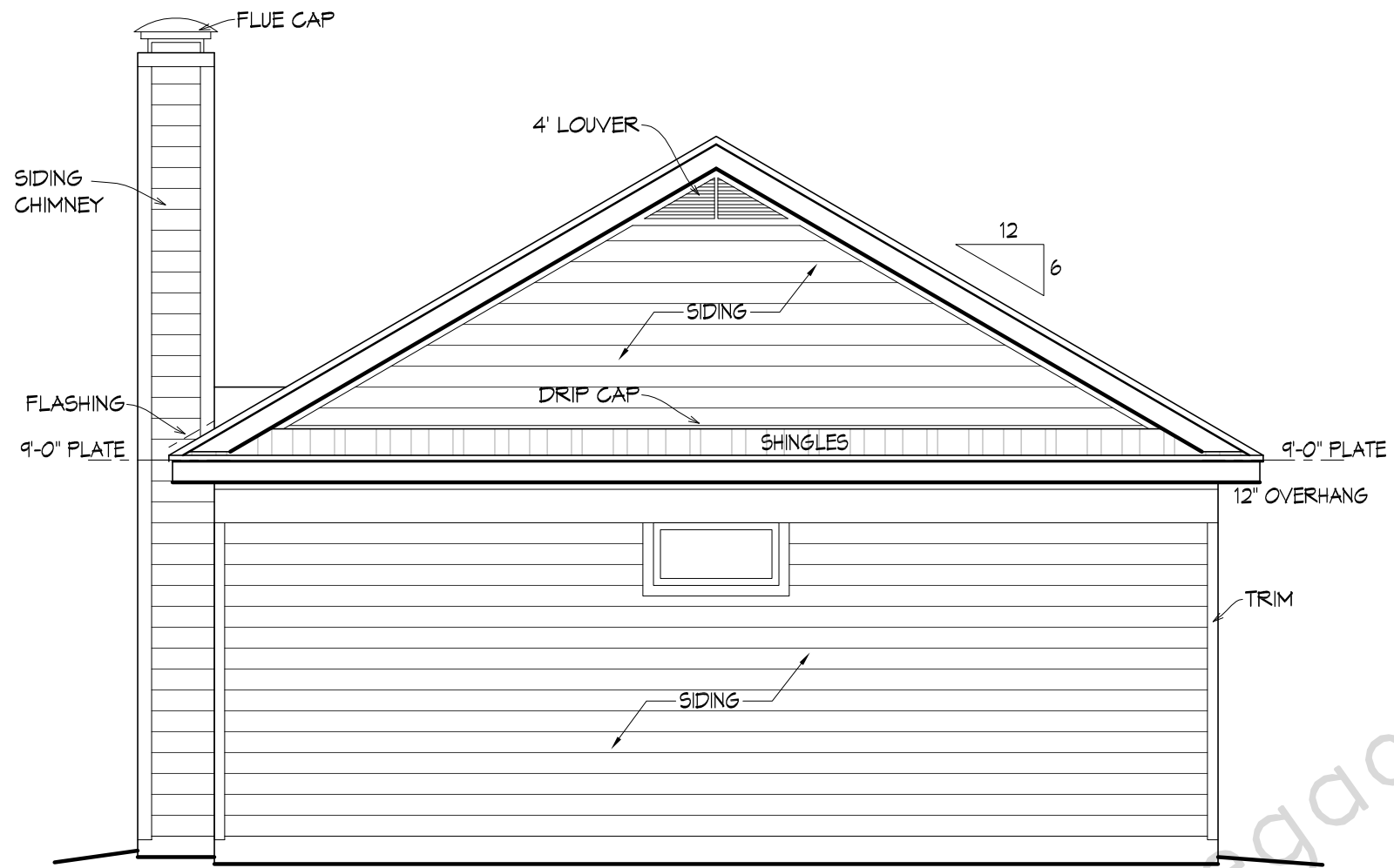
SCALE: 1/4" = 1'-0" REAR ELEVATION
