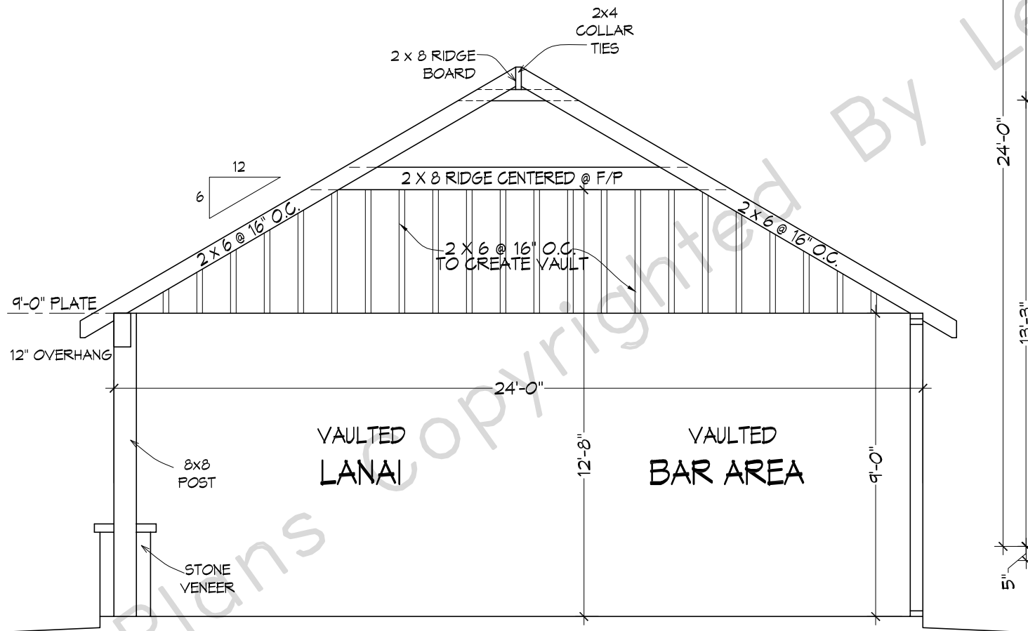
MAIN BODY SECTION SCALE: 1/4" = 1'-0"
