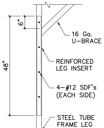
*** REINFORCED LEG INSERT (LEG HEIGHTS >12' TO 14')
