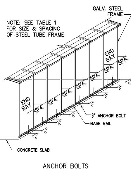
1/3 SOIL BASE RAIL ANCHOR DETAIL
