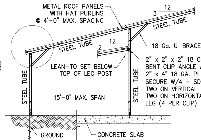
TYPICAL SIDE EXTENSION SECTION
