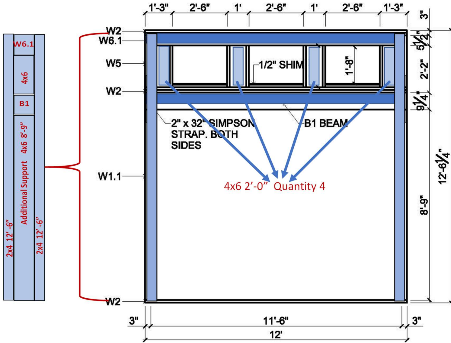
CENTER WALL FRAMING PLAN
