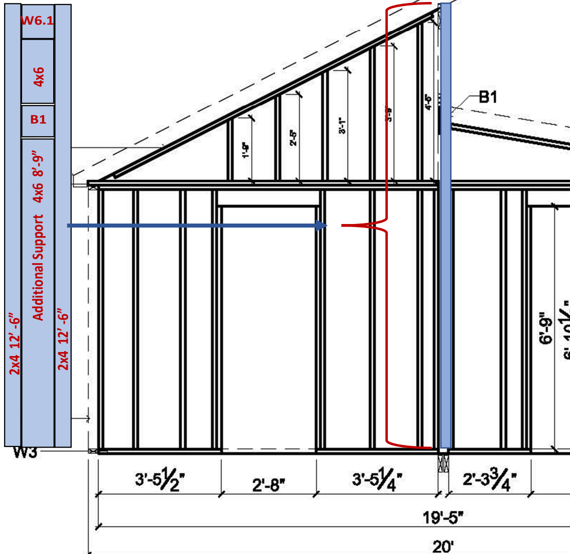
FRONT WALL FRAMING PLAN
