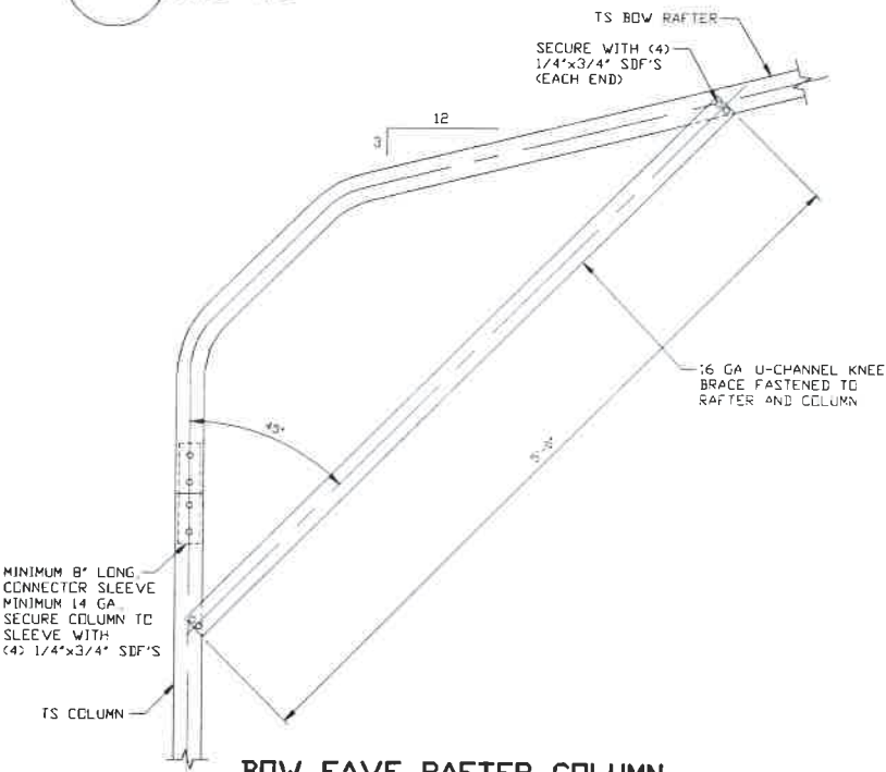
BOW EAVE RAFTER COLUMN CONNECTION DETAIL HEIGHTS 10'-0" < TO ≤ 12'-0" @ 4'-0" O.C. SCALE: NTS
