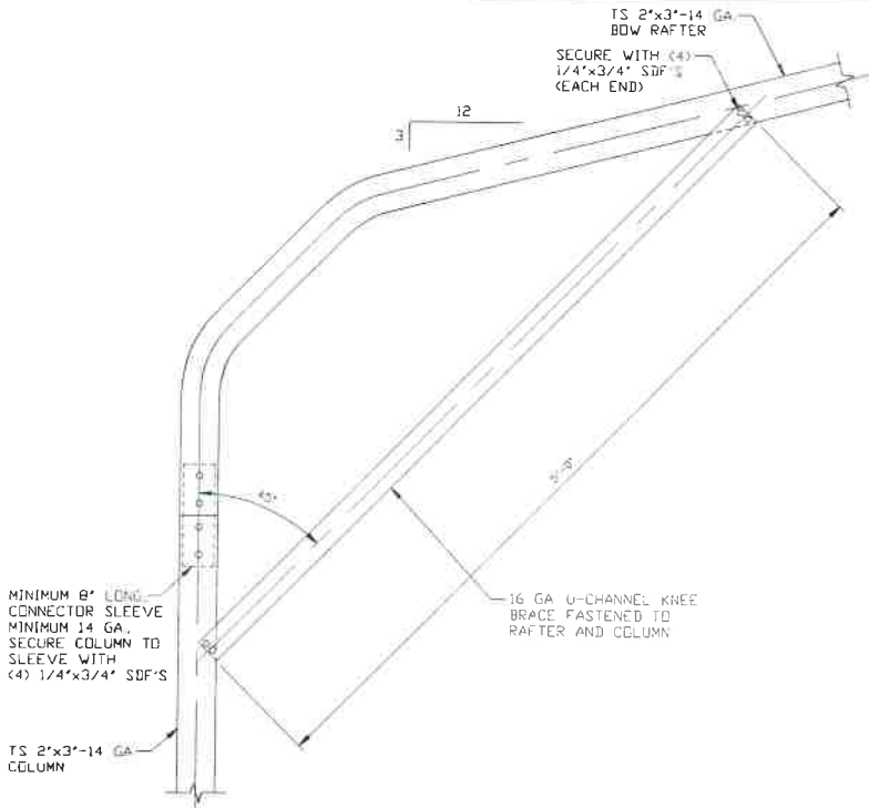
BOW RAFTER COLUMN CONNECTION DETAIL HEIGHTS 12'-0" < TO ≤ 14'-0" @ 4'-0" O.C. SCALE: NTS
