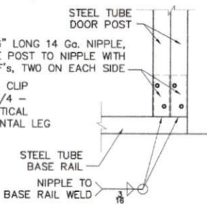
6 POST/BASE RAIL DETAIL
