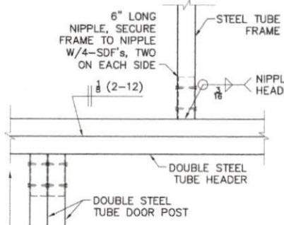
7 SIDE HEADER DETAIL (DOUBLE HEADER FOR 8' TO 16' OPENING)
