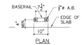
9 VERTICAL PANEL ATTACHMENT
