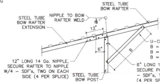
2 BOW/POST DETAIL
