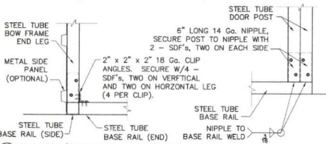
3 END BOW/BASE RAIL CONNECTION
