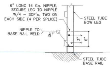
6 BOW/BASE RAIL CONNECTION DETAIL
