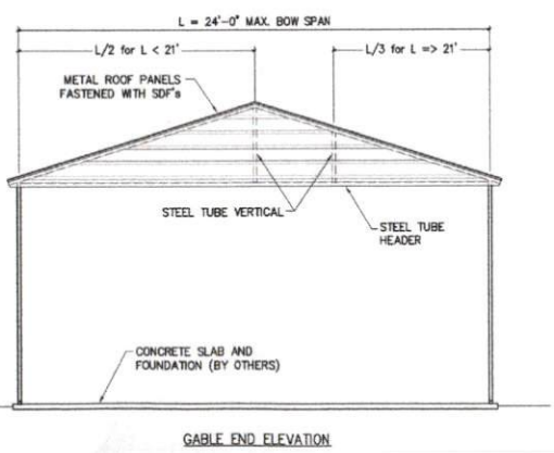
GABLE END ELEVATION
