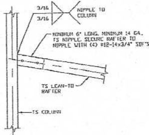
16A LEAN-TO RAFTER TO RAFTER POST CONNECTION DETAIL FOR WIDTHS \le 12'-0'' SCALE: NTS
