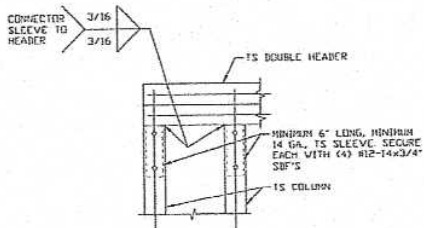
8 DOUBLE HEADER/COLUMN CONNECTION DETAIL
