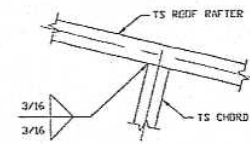
11 RAFTER TO CHORD CONNECTION DETAIL
