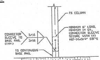
3B POST/BASE RAIL CONNECTION DETAIL SCALE: NTS
