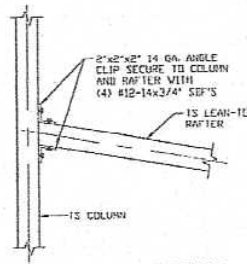
16B LEAN-TO RAFTER TO RAFTER POST CONNECTION DETAIL FOR WIDTHS \le 12'-0'' SCALE: NTS
