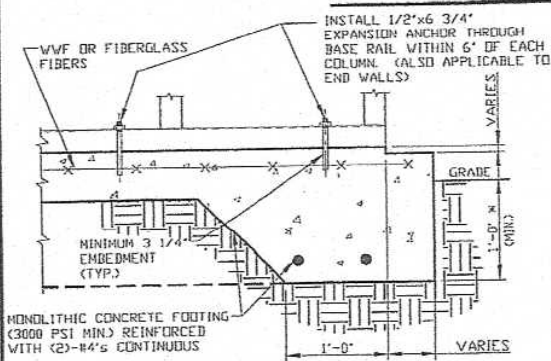
2A CONCRETE MONOLITHIC SLAB BASE RAIL ANCHORAGE SCALE: NTS MINIMUM ANCHOR EDGE DISTANCE IS 4" X COORDINATE WITH LOCAL CODES/ORD.
