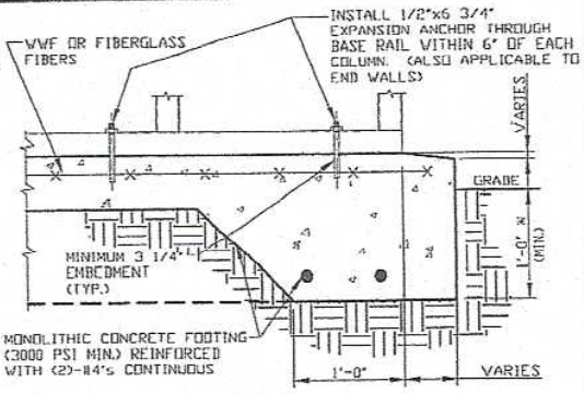
2B CONCRETE SLAB BASE RAIL ANCHORAGE SCALE: NTS MINIMUM ANCHOR EDGE DISTANCE IS 4" X COORDINATE WITH LOCAL CODES/ORD.
