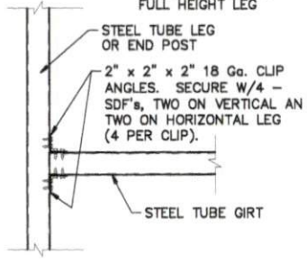
4 GIRT TO POST CONNECTION
