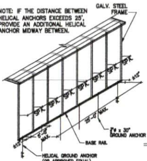
HELICAL GROUND ANCHORS
