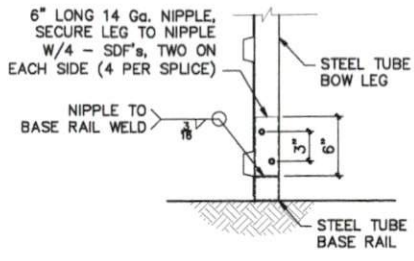
6 BOW/BASE RAIL CONNECTION DETAIL
