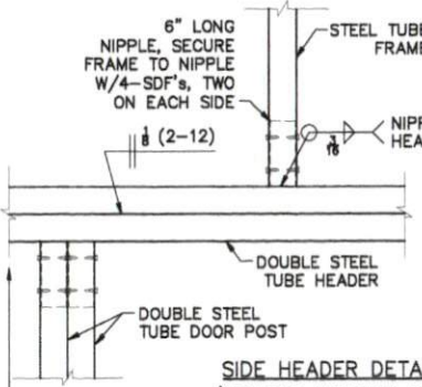
SIDE HEADER DETAIL (DOUBLE HEADER FOR 8' TO 16' OPENING)
