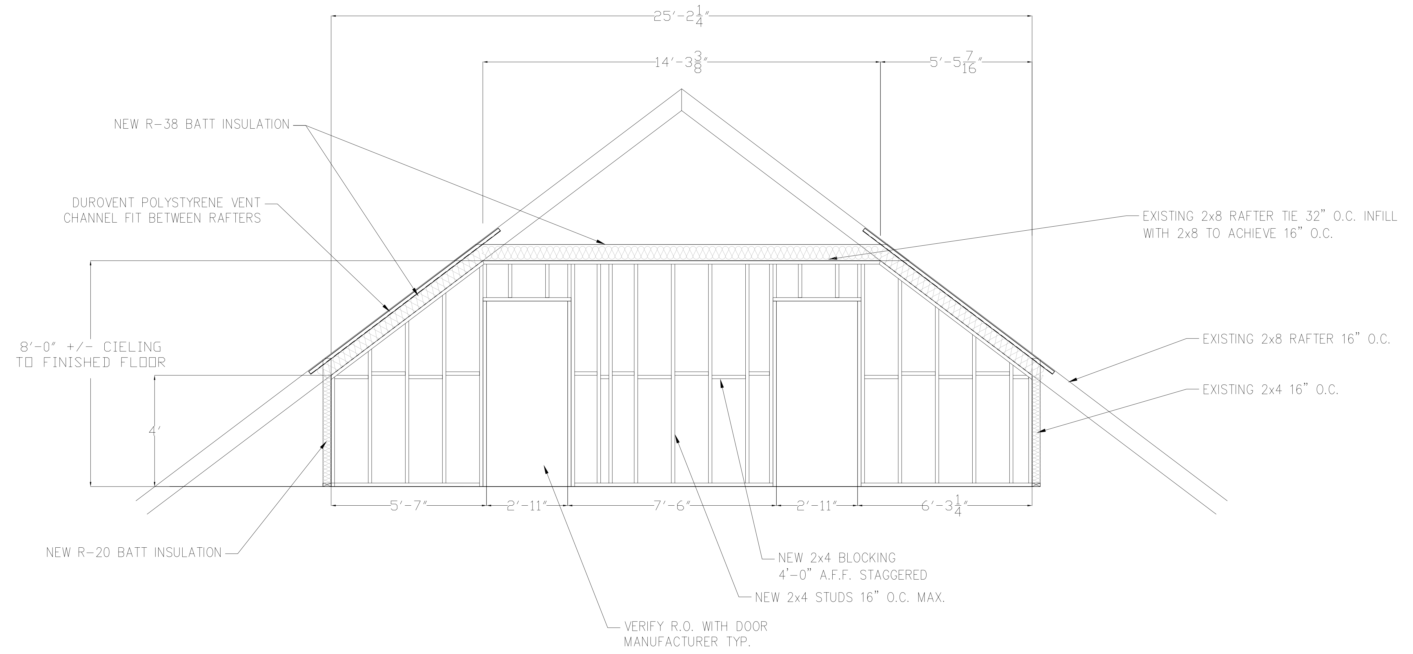
1 SECTION 1/4" = 1'-0"
