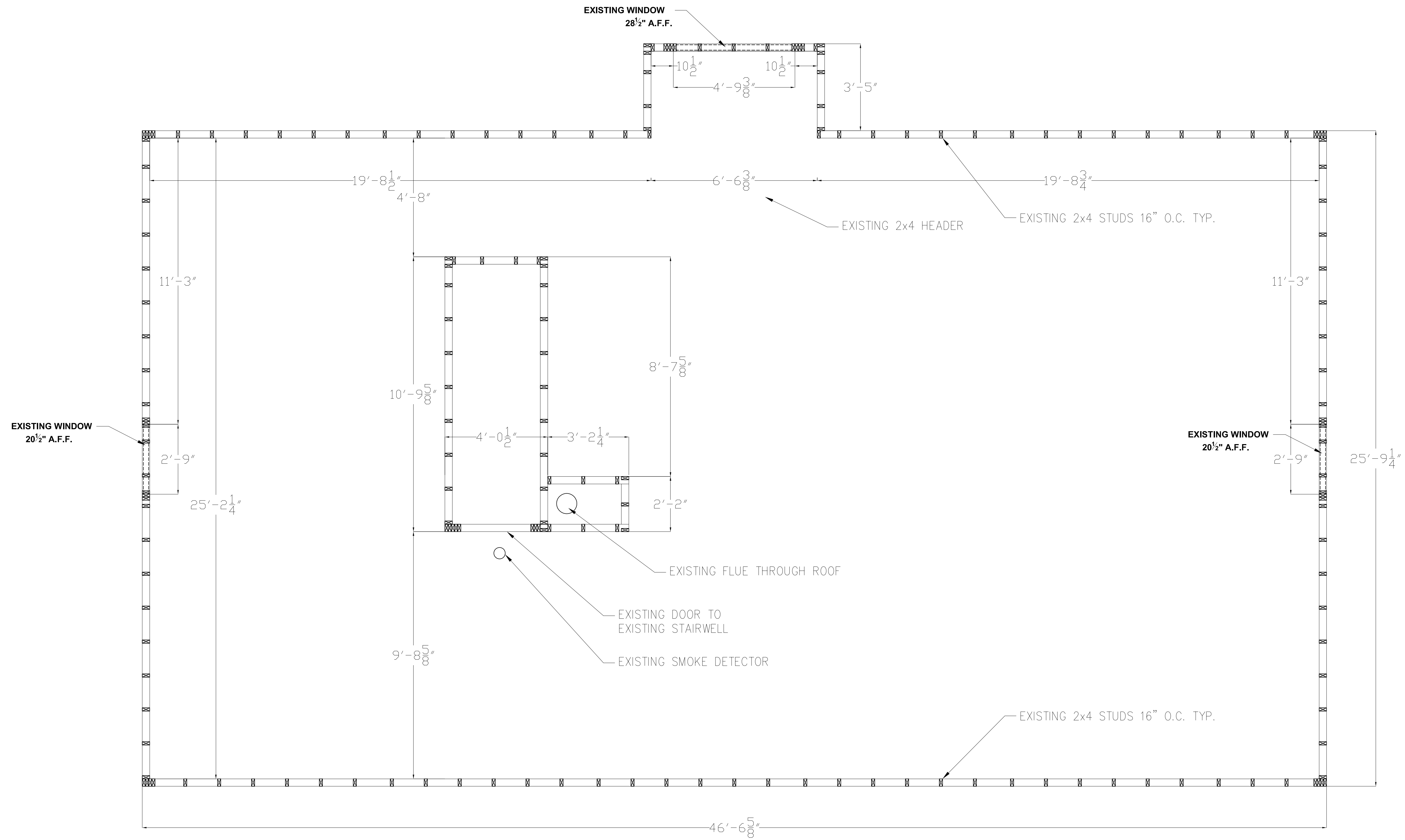
1 EXISTING SECOND FLOOR PLAN 1/4" = 1'-0"
