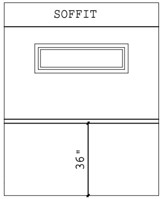
CABINET ELEVATION J BEHIND MBH TUB
