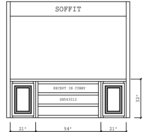
CABINET ELEVATION I ETC
