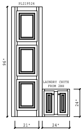
CABINET ELEVATION G PANTRY/LAUNDRY CHUTE 2BH
