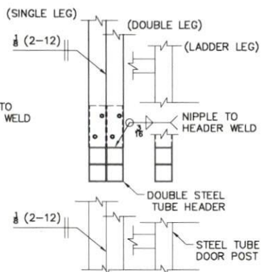
8 HEADER SECTION (ONE HEADER FOR SINGLE LEG, TWO HEADERS FOR DOUBLE LEG AND LADDER LEG)
