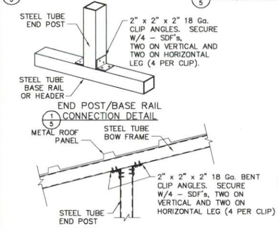
1 END POST/BASE RAIL CONNECTION DETAIL
