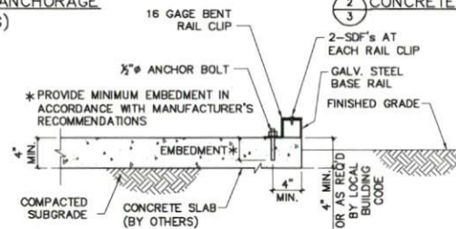
ALTERNATE BASE RAIL ANCHORAGE
