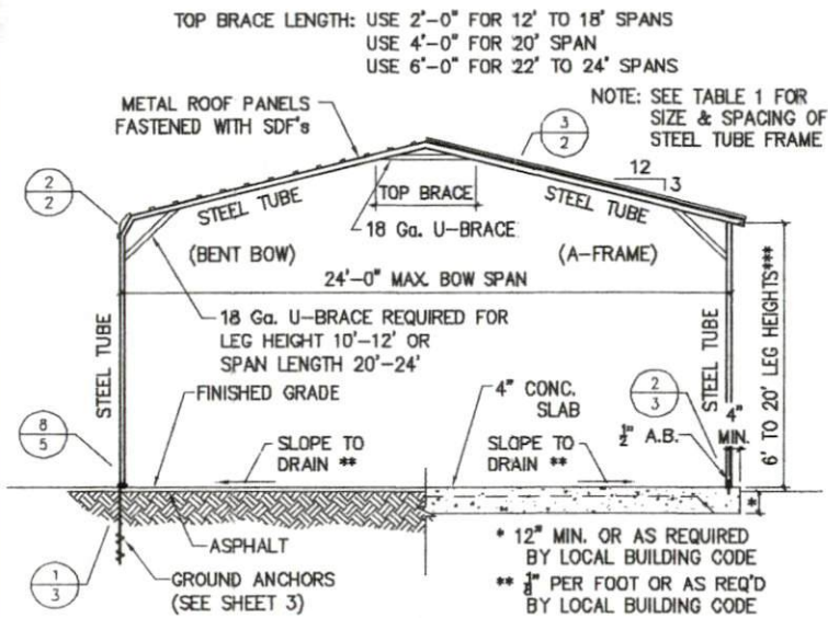
1/2 TYPICAL BOW SECTION
