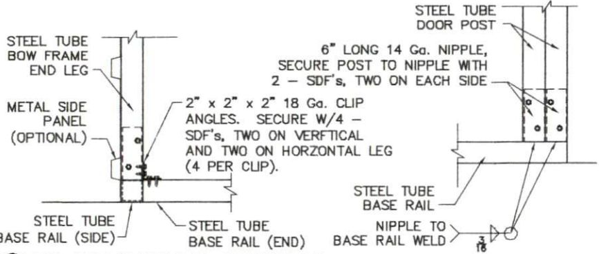
3 END BOW/BASE RAIL CONNECTION
