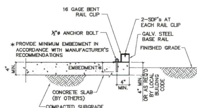
2 ALTERNATE BASE RAIL ANCHORAGE
