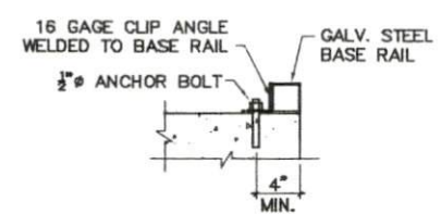
ALTERNATE BASE RAIL CLIP
