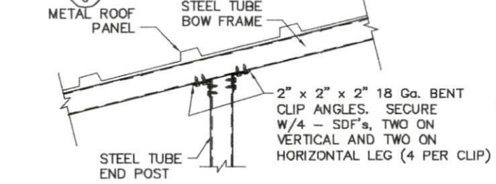
2 END POST TO BOW FRAME CONNECTION
