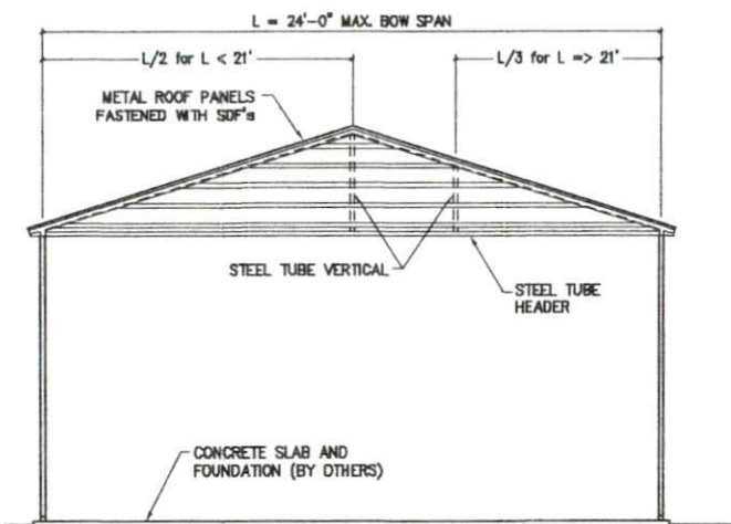
GABLE END ELEVATION
