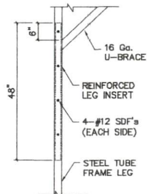
*** REINFORCED LEG INSERT (LEG HEIGHTS >12' to 14')
