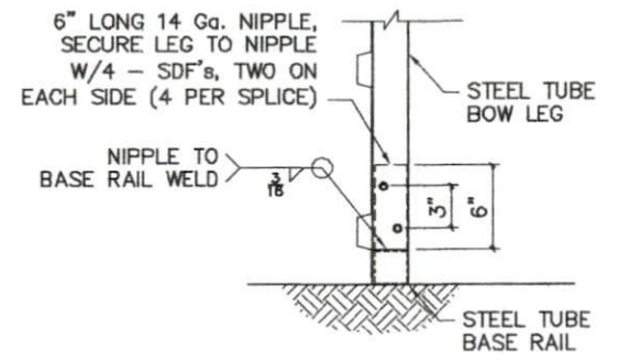
6 BOW/BASE RAIL CONNECTION DETAIL
