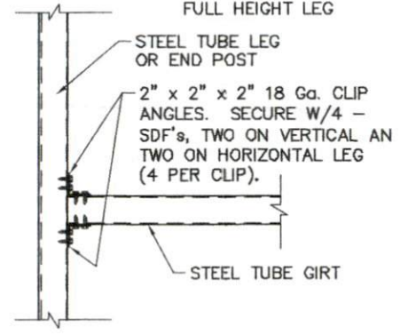
4 GIRT TO POST CONNECTION
