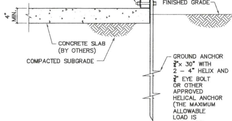
2 ALTERNATE BASE RAIL ANCHORAGE
