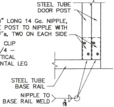
6 POST/BASE RAIL DETAIL
