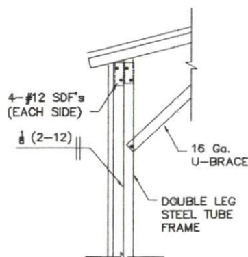
*** DOUBLE LEG (LEG HEIGHTS >12' to 16')
