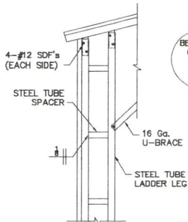
*** LADDER LEG (LEG HEIGHTS 16' to 20')
