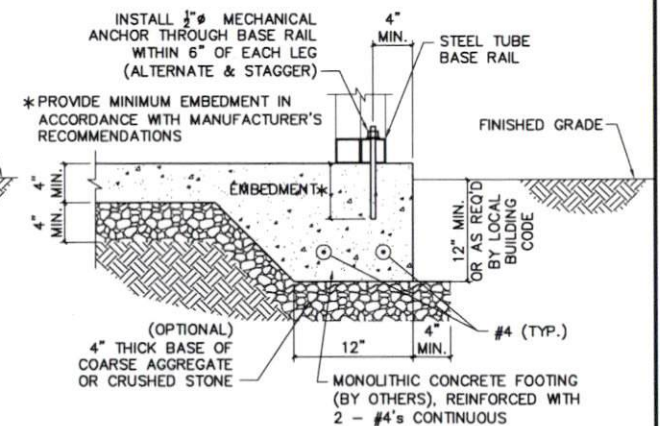
2/3 CONCRETE BASE RAIL ANCHORAGE (DOUBLE LEG)
