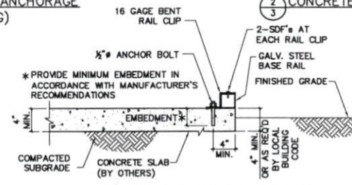
2/3 ALTERNATE BASE RAIL ANCHORAGE
