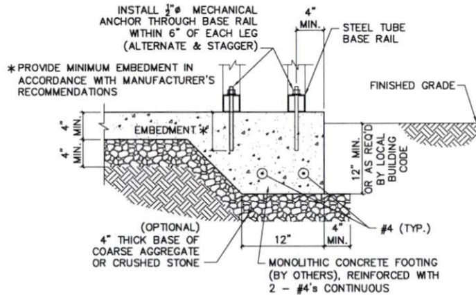
2/3 CONCRETE BASE RAIL ANCHORAGE (LADDER LEG)
