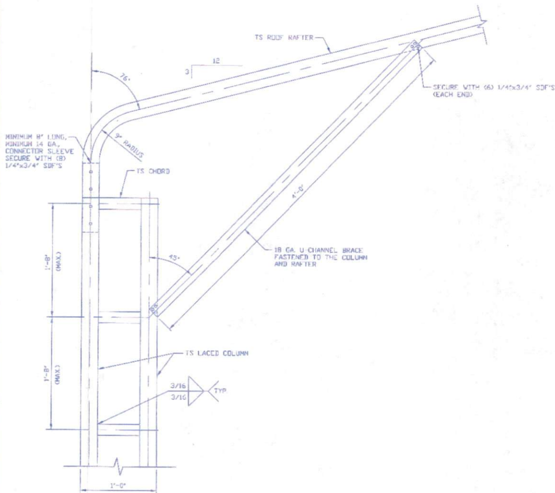
1A BOX EAVE RAFTER/CORNER POST CONNECTION DETAIL FOR HEIGHTS 16'-0" < TO ≤ 20'-0" SCALE: NTS
