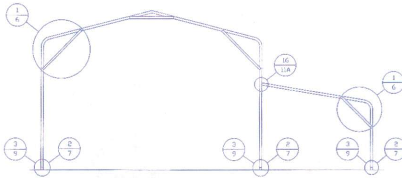
TYPICAL BOW EAVE RAFTER LEAN-TO OPTIONS FRAMING SECTION SCALE: NTS
