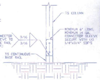
3C POST/BASE RAIL CONNECTION DETAIL SCALE: NTS
