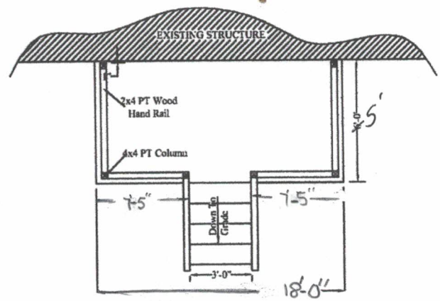
FLOOR PLAN Scale: 1/4" = 1'-0"
