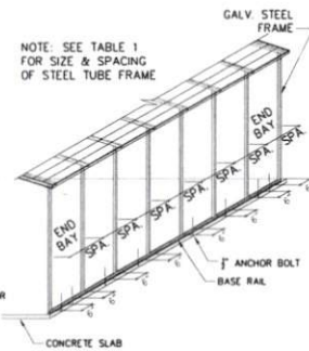
ANCHOR BOLTS
