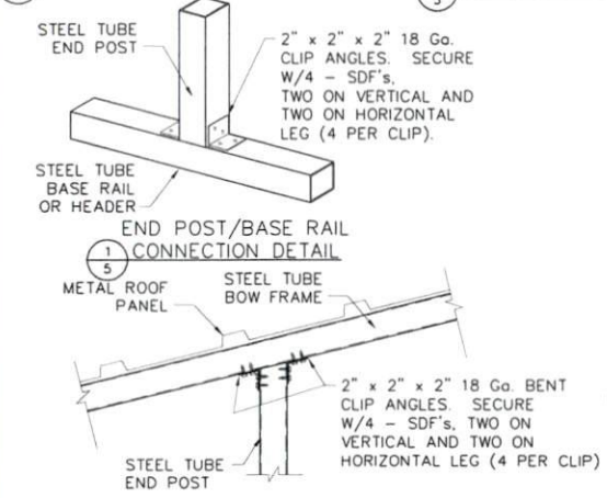
2 END POST TO BOW FRAME CONNECTION
