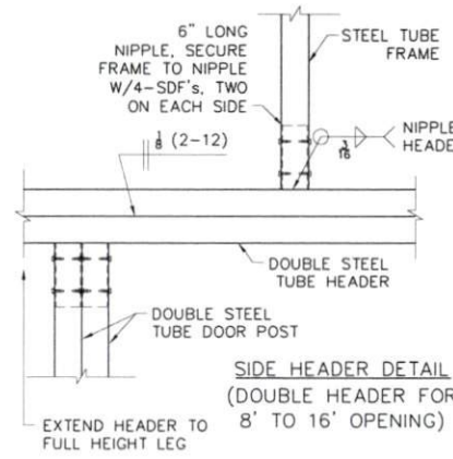
7 BOW / HEADER DETAIL
