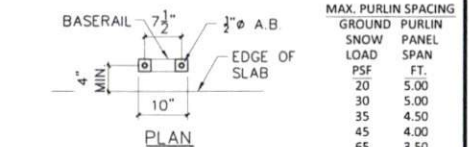
VERTICAL PANEL ATTACHMENT
