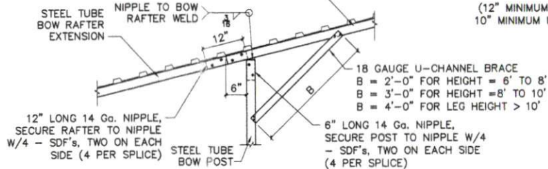
BOW/POST DETAIL
