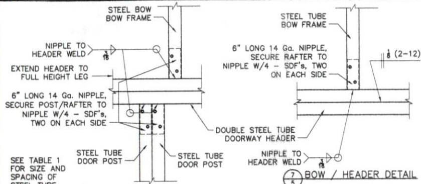
5 BOW FRAME/HEADER DETAIL
