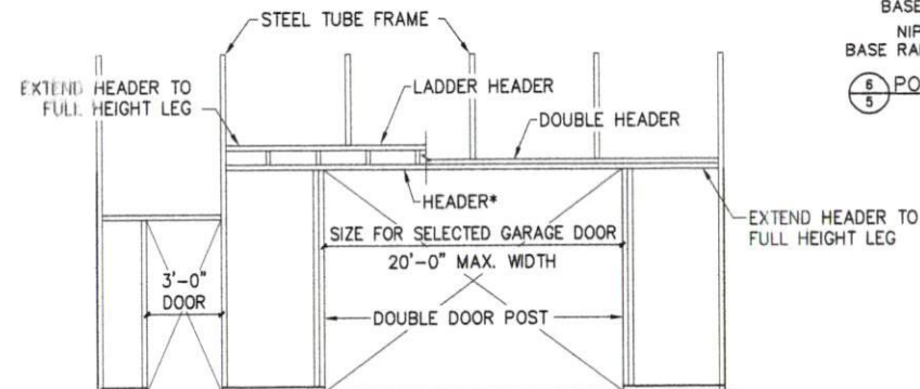
SIDE OPENING
