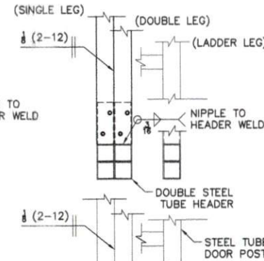
HEADER SECTION
