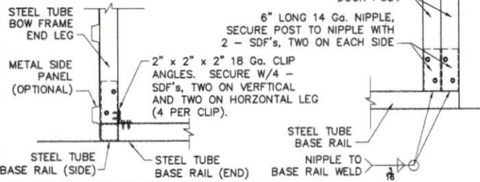
3 END BOW/BASE RAIL CONNECTION
