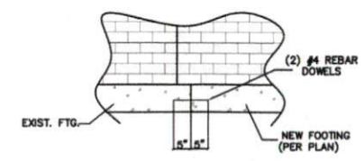
A NEW TO EXISTING FOOTING DETAIL
