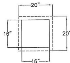
FOOTING/MORTAR BLOCK DETAIL
