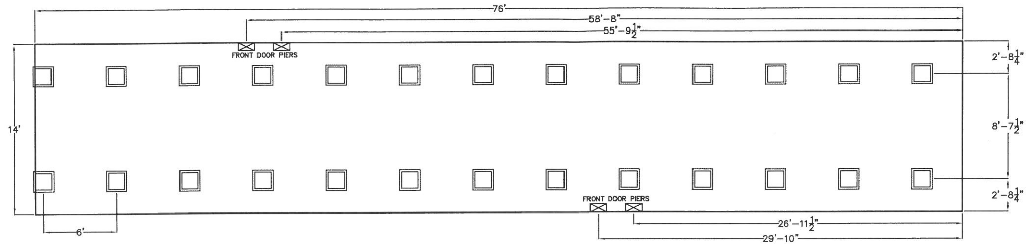
TRAILER FOOTING PLAN SCALE: 1"=60'
