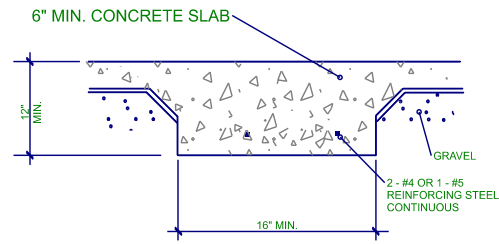
INTEGRAL SLAB FOOTING DETAIL 1.2 N.T.S.
