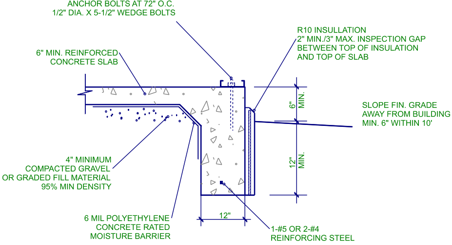
MONOLITHIC SLAB DETAIL 1.1 N.T.S.
