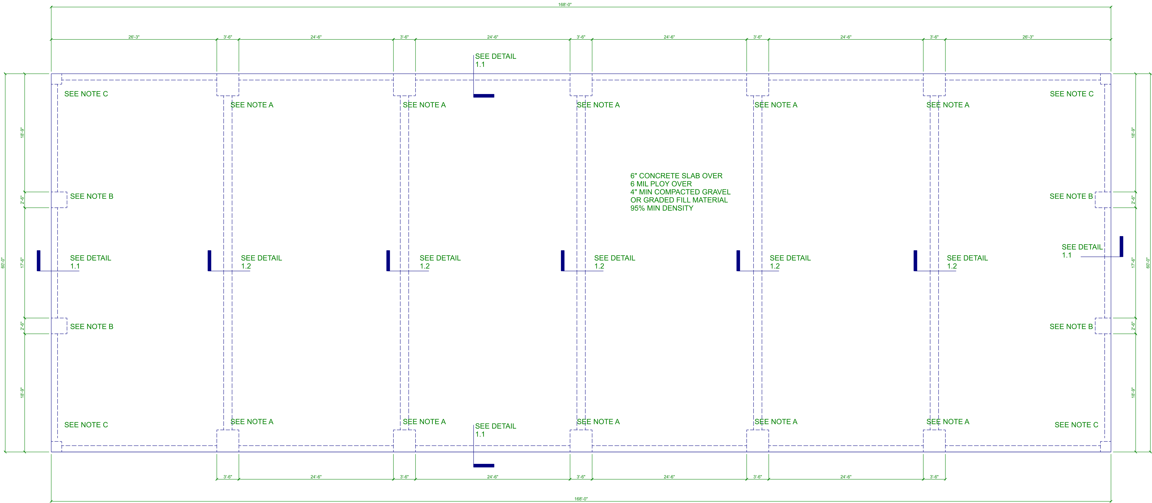
FOUNDATION PLAN SCALE: 1/8" = 1'
