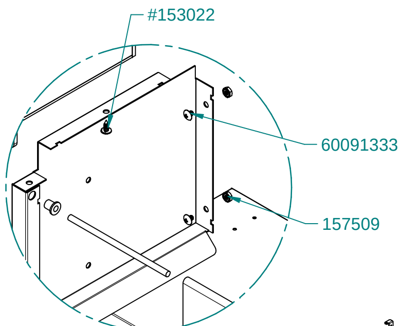
DETAIL B
