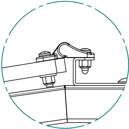
DETAIL D
