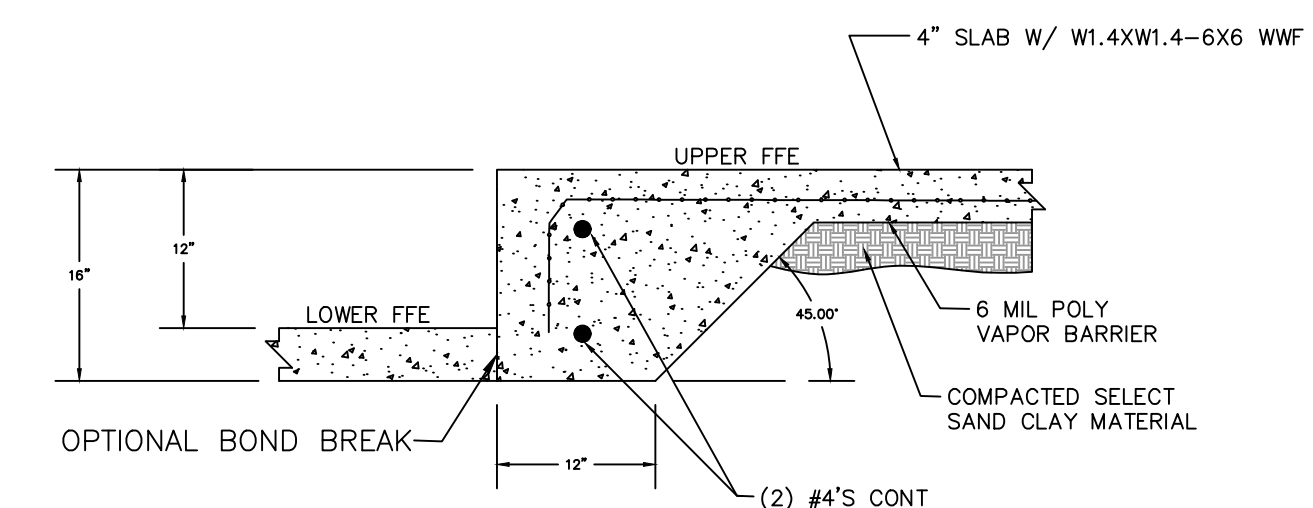
SECTION C CONT. FOOTING DETAIL
