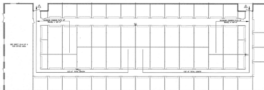
LIFE SAFETY PLAN BUILDING "1" SCALE 1/8" = 1'-0"
