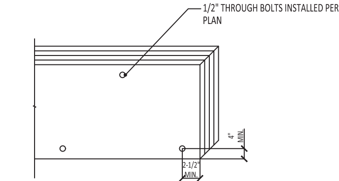
4 D-2f MULTI-PLY BEAM FASTENING DETAIL SEE NOTES ON PLAN FOR MORE INFO
