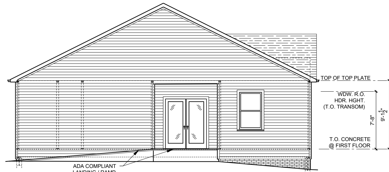
3 REAR ELEVATION 1/8" = 1'-0"
