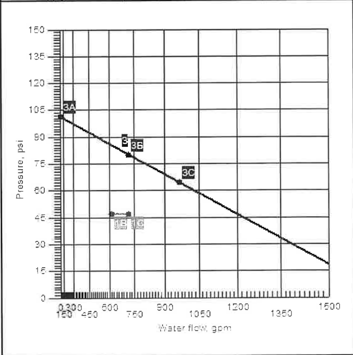
Altis Fire Sprinkler Uprights Water Supply at Node 14 (969.00, 0.00, 101.800, 64.900)
