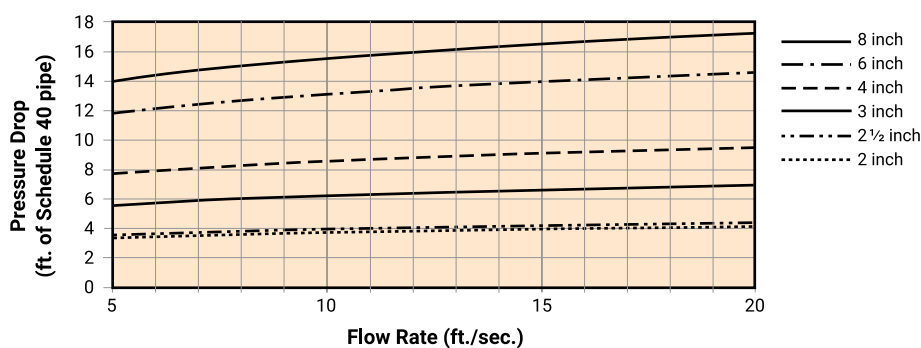
ST-1 90° Tee Short Pattern Fitting - Pressure Drop
