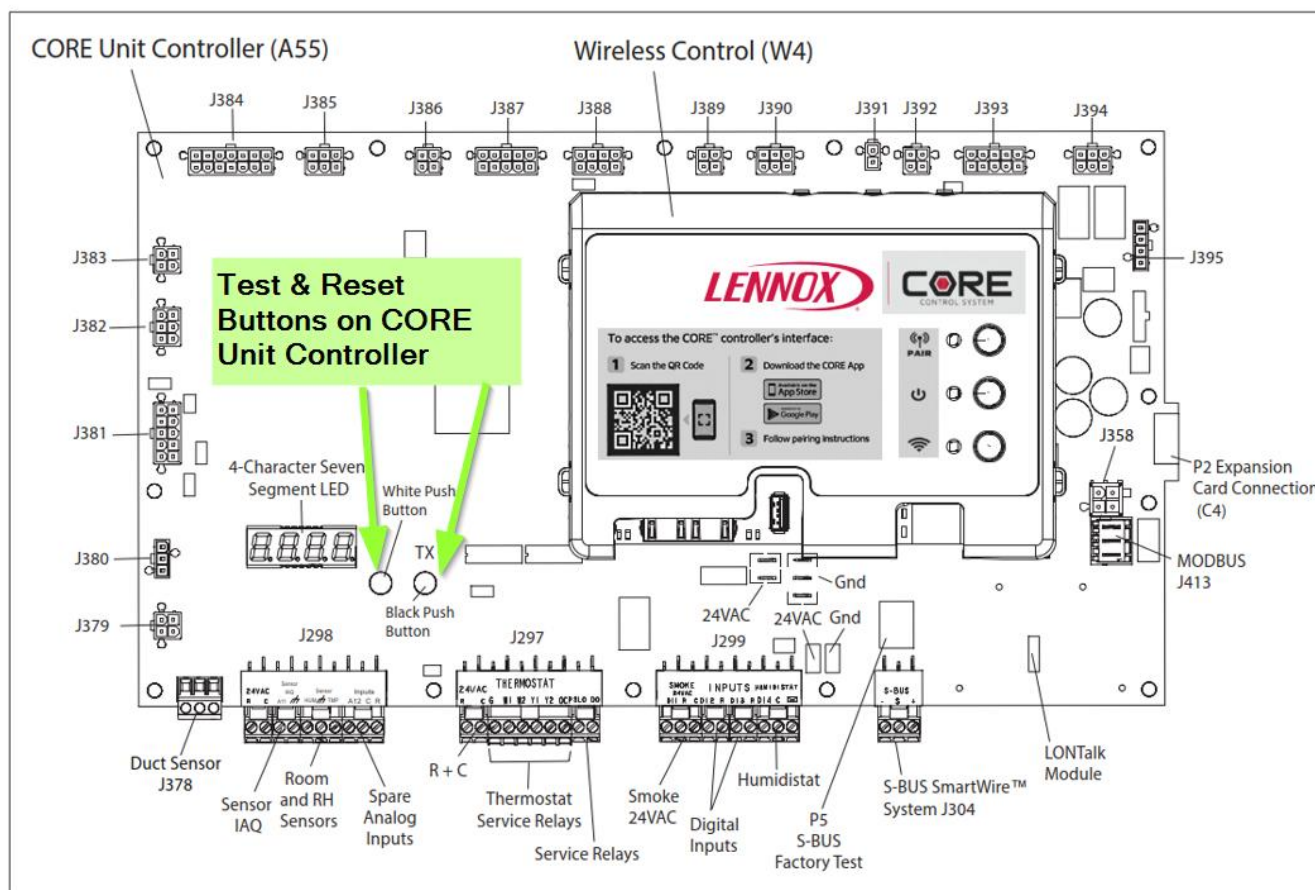
Figure 2. Push Buttons
