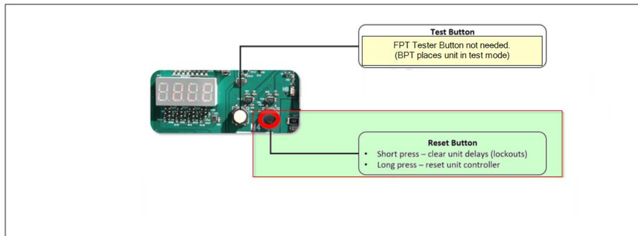
Figure 2. Push Buttons
