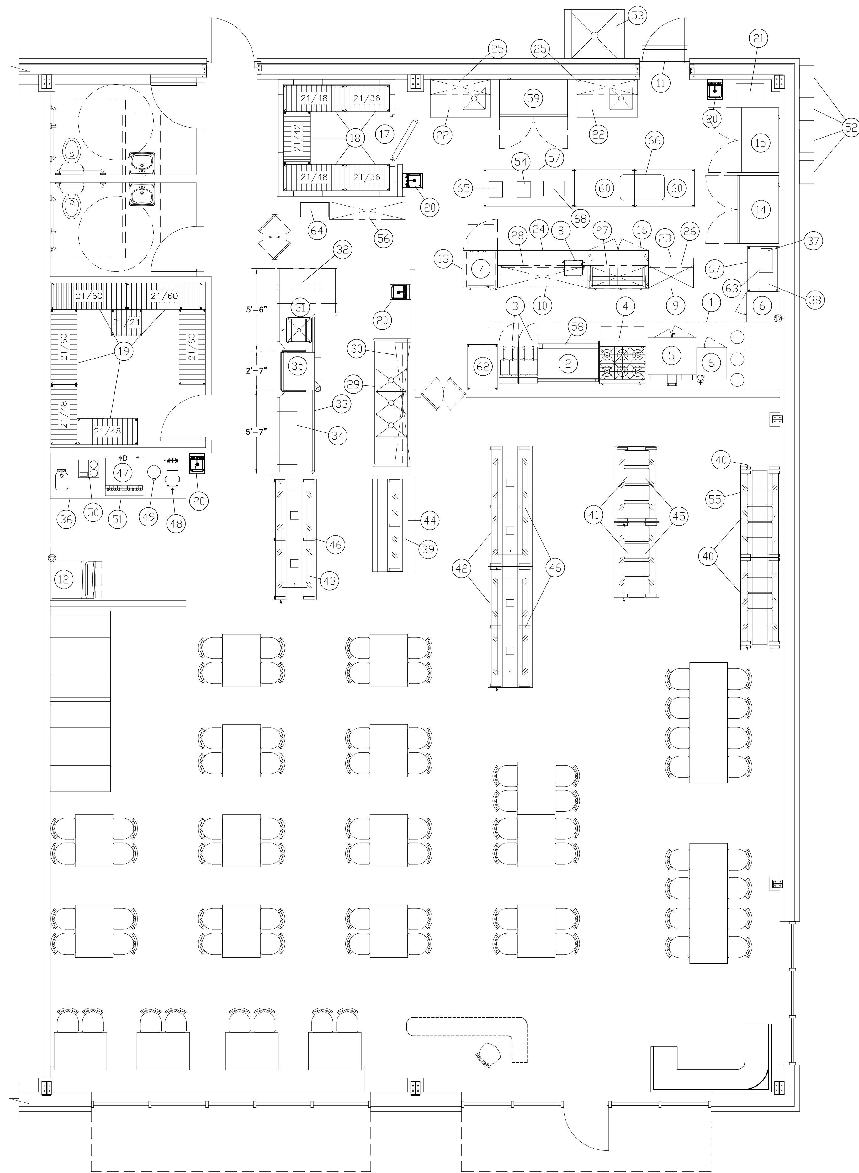
EQUIPMENT PLAN SCALE: 1/4" = 1'-0"
