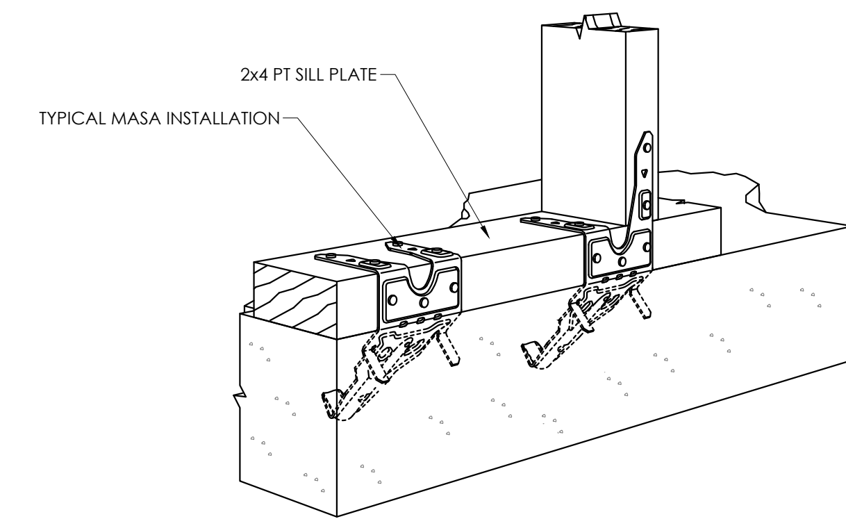
8 PERSPECTIVE OF MASA INSTALLATION SCALE: NONE
