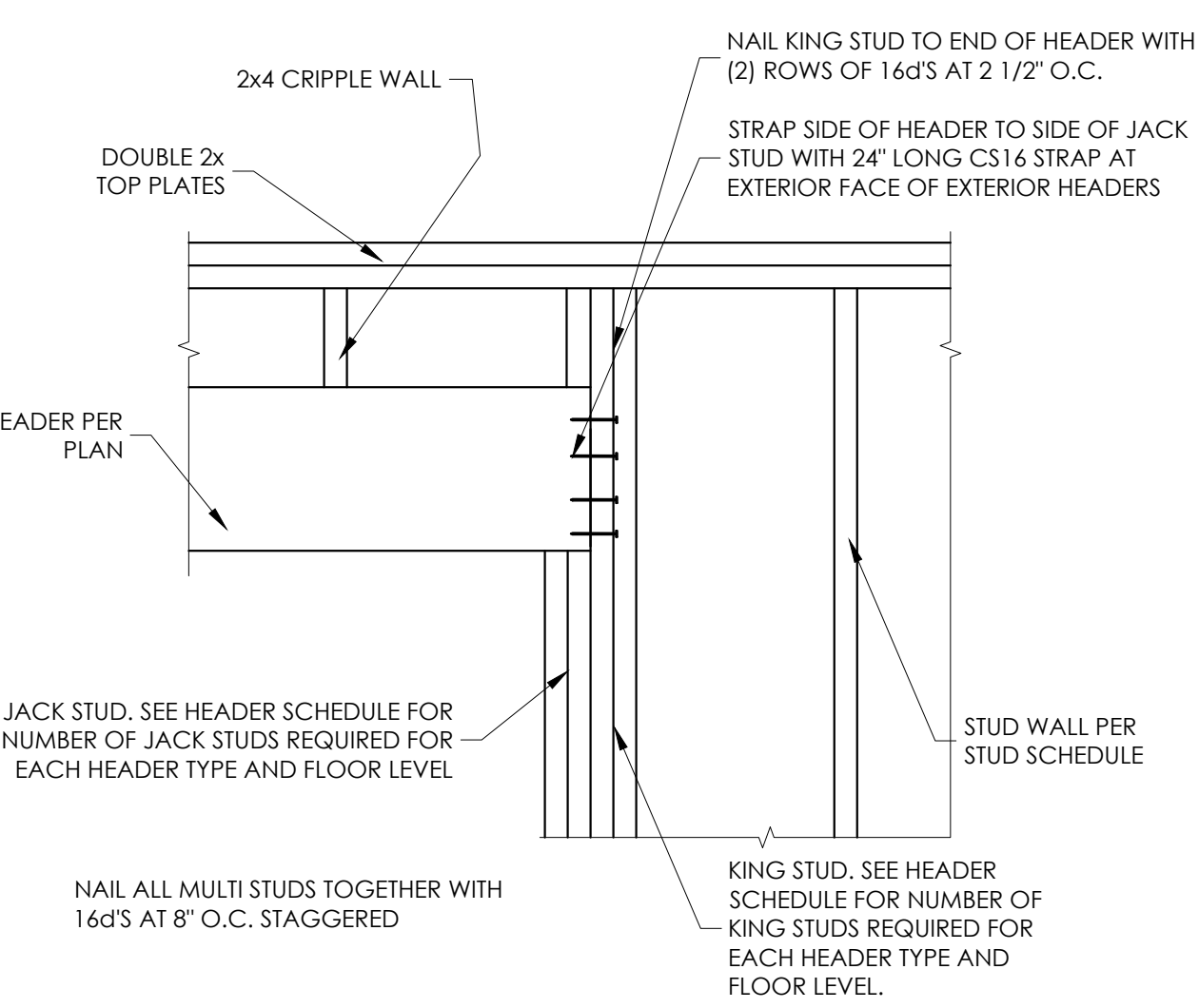
10 HEADER BEARING DETAIL SCALE: NONE
