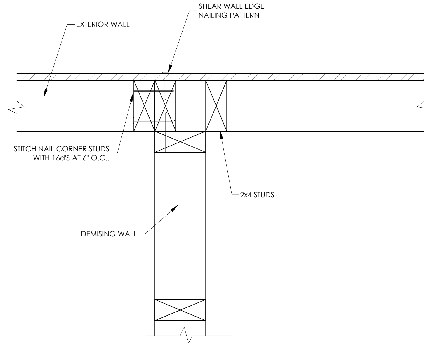
11 DEMISING WALL TO EXTERIOR WALL SCALE: NONE
