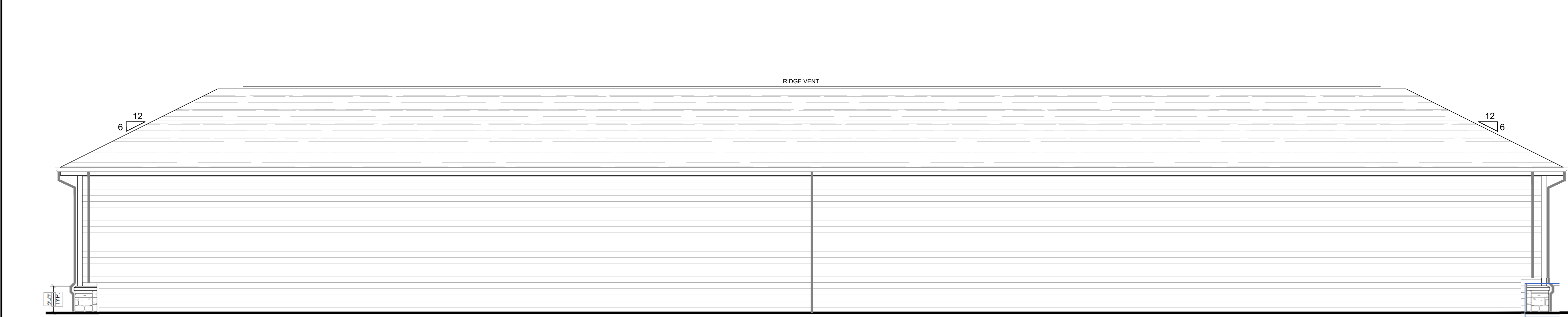
4 GARAGE TYPE 1 - REAR ELEVATION SCALE: 1/4" = 1'-0"
