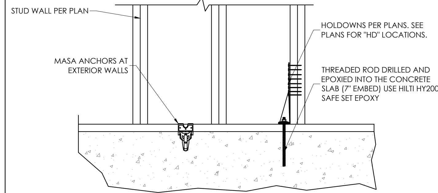
7 ELEVATION OF WALL ANCHORAGE SCALE: NONE
