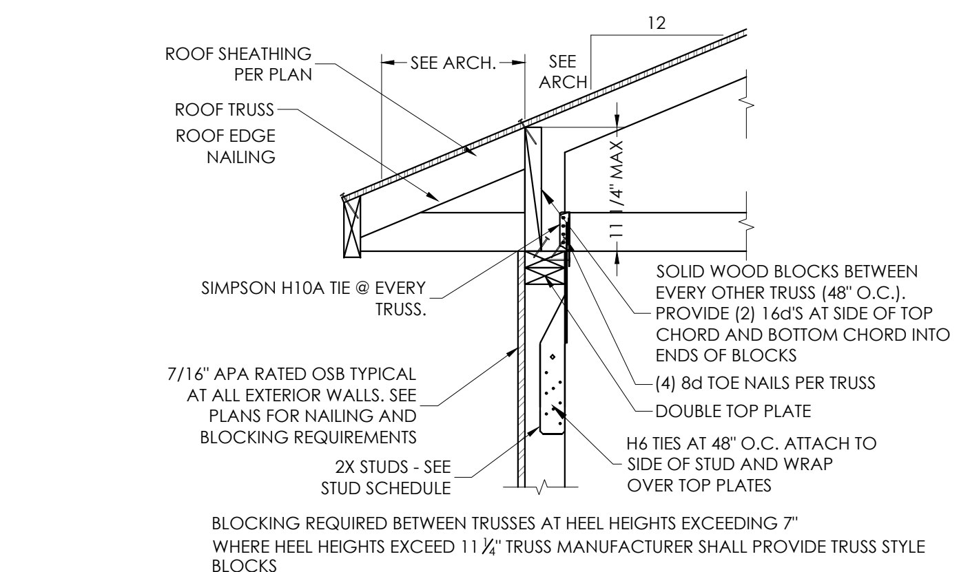
8 ROOF TRUSS CONNECTION AT EXTERIOR WALL SCALE: NONE
