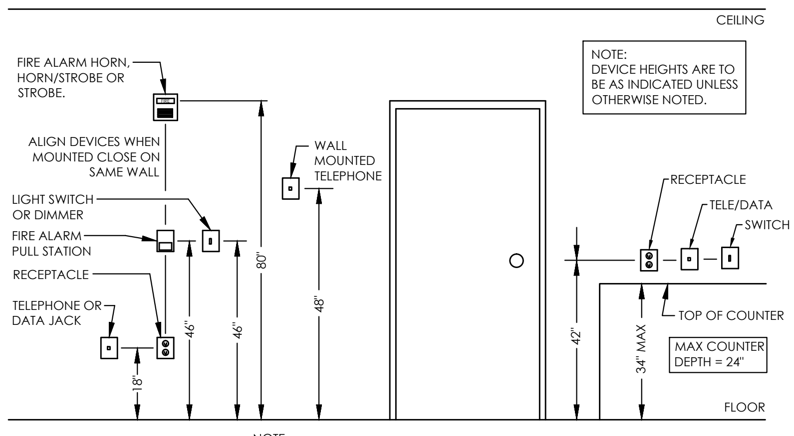
1 TYPICAL DEVICE MOUNTING HEIGHTS NO SCALE
