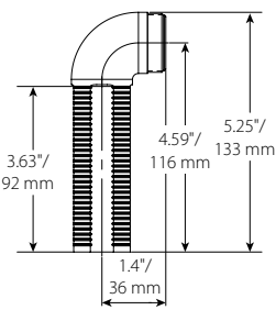
Long 90° Low-Profile Elbow Reducer
