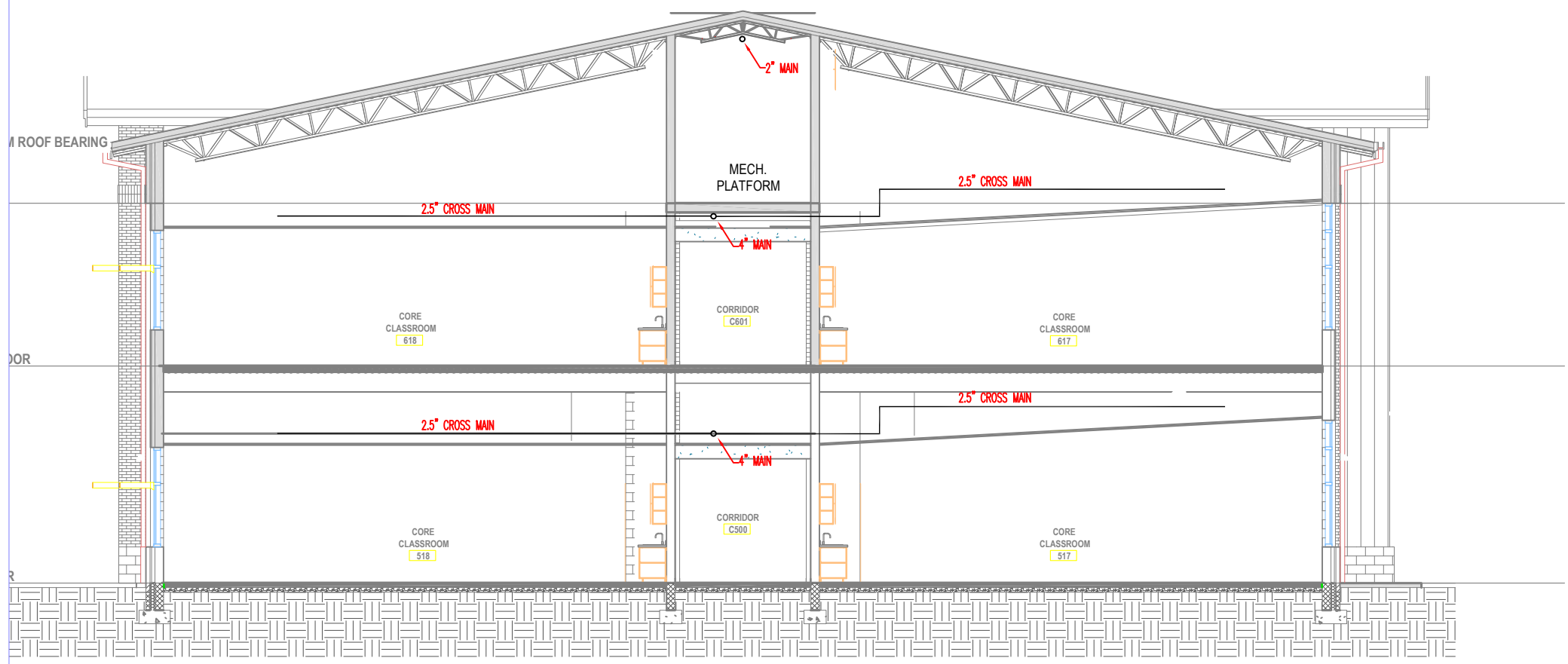
AREA 500 - SECTION SCALE: 3/32" = 1'-0"
