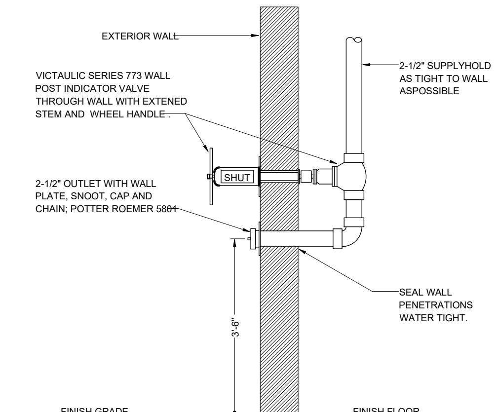
FIRE HOSE VALVE CONNECTION NO SCALE
