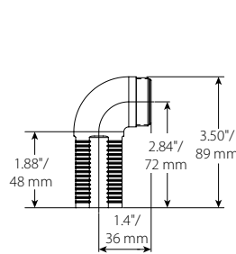
Short 90° Low-Profile Elbow Reducer
