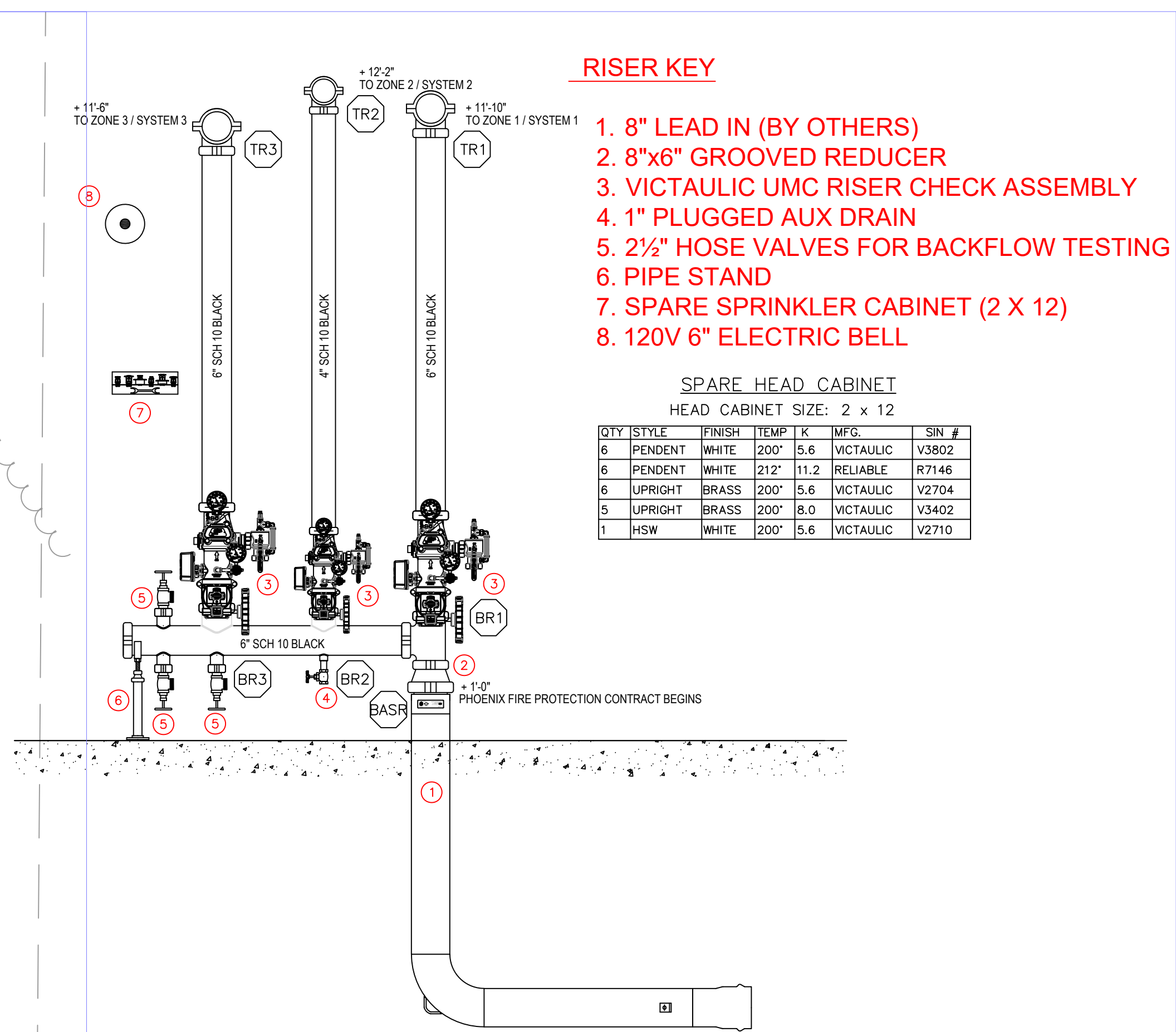
RISER DETAIL
