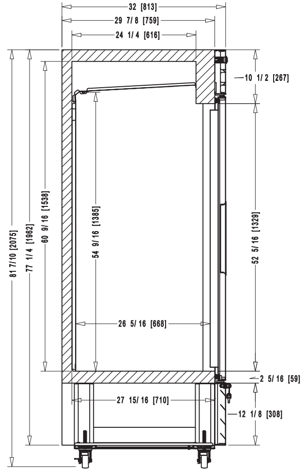
SIDE VIEW
