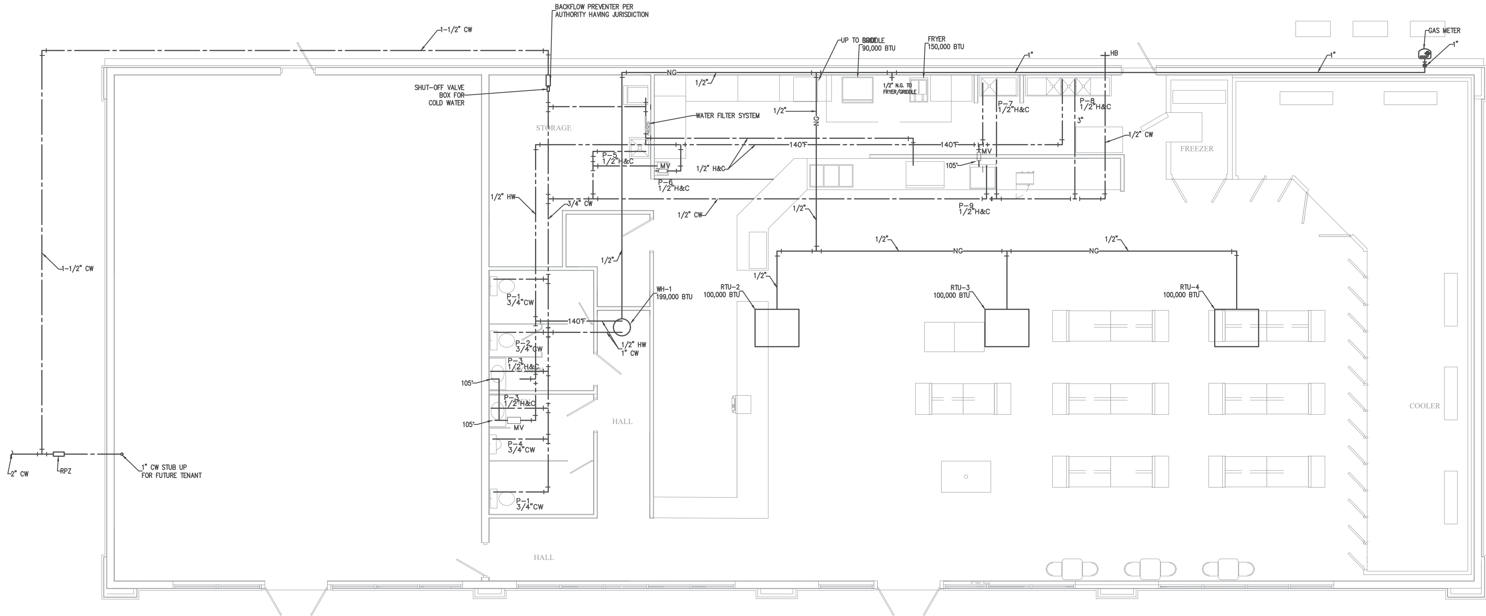
1 P3 WATER PLAN 3/16"=1'-0"
