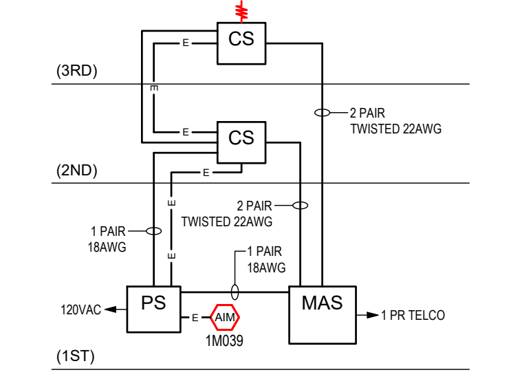
2 AOR/2-WAY COMM. SYSTEM RISER FA-4 Scale: None
