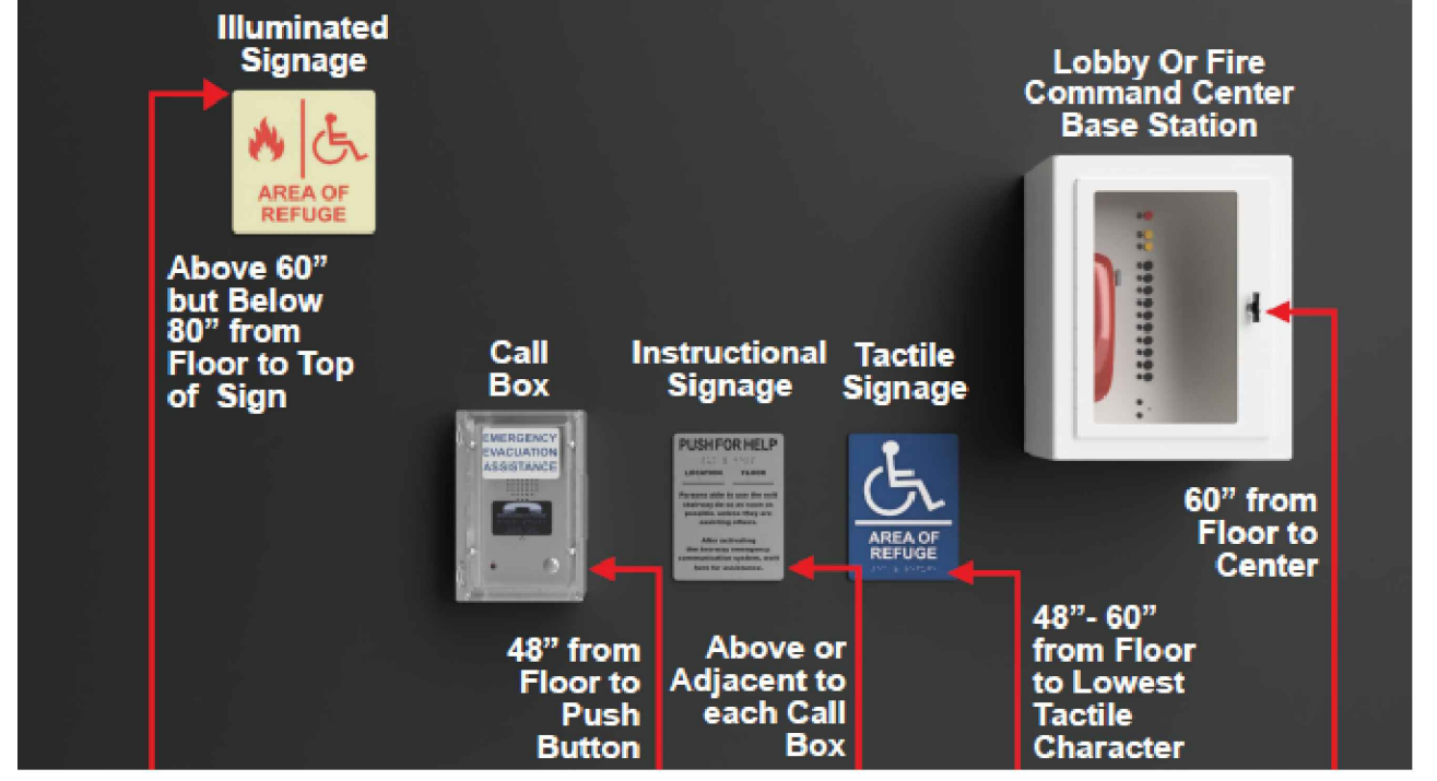
3 AOR/2-WAY COMM. MOUNTING HEIGHTS FA-4 Scale: None
