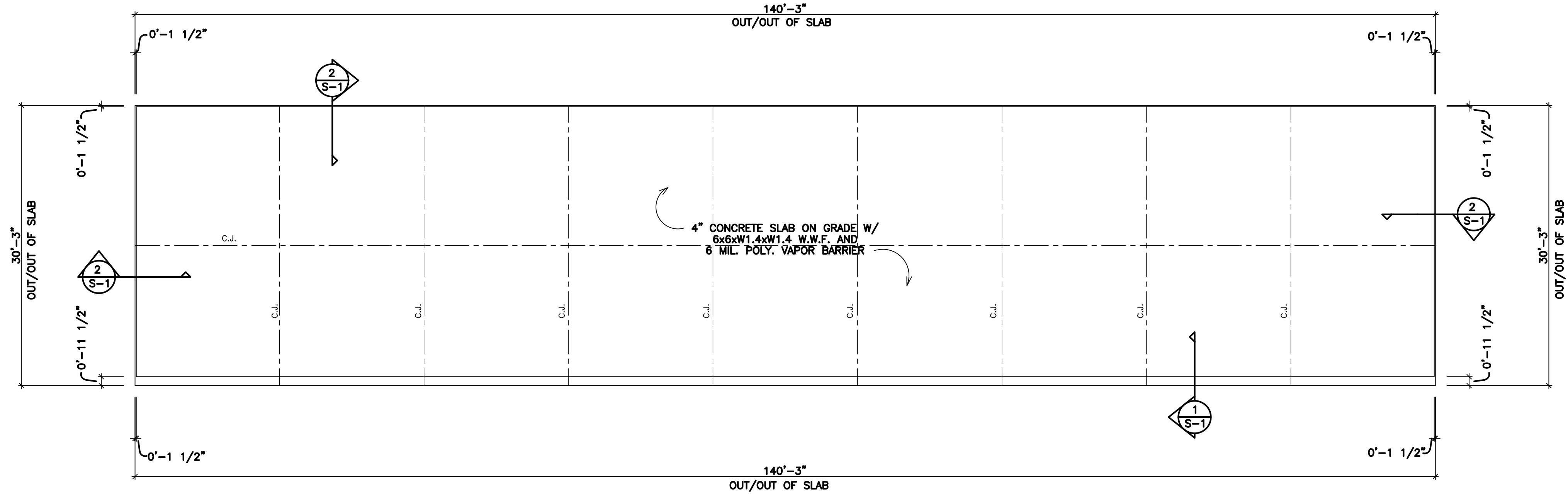
FOUNDATION PLAN – BLDG S4 SCALE: 1/8" = 1'-0"
