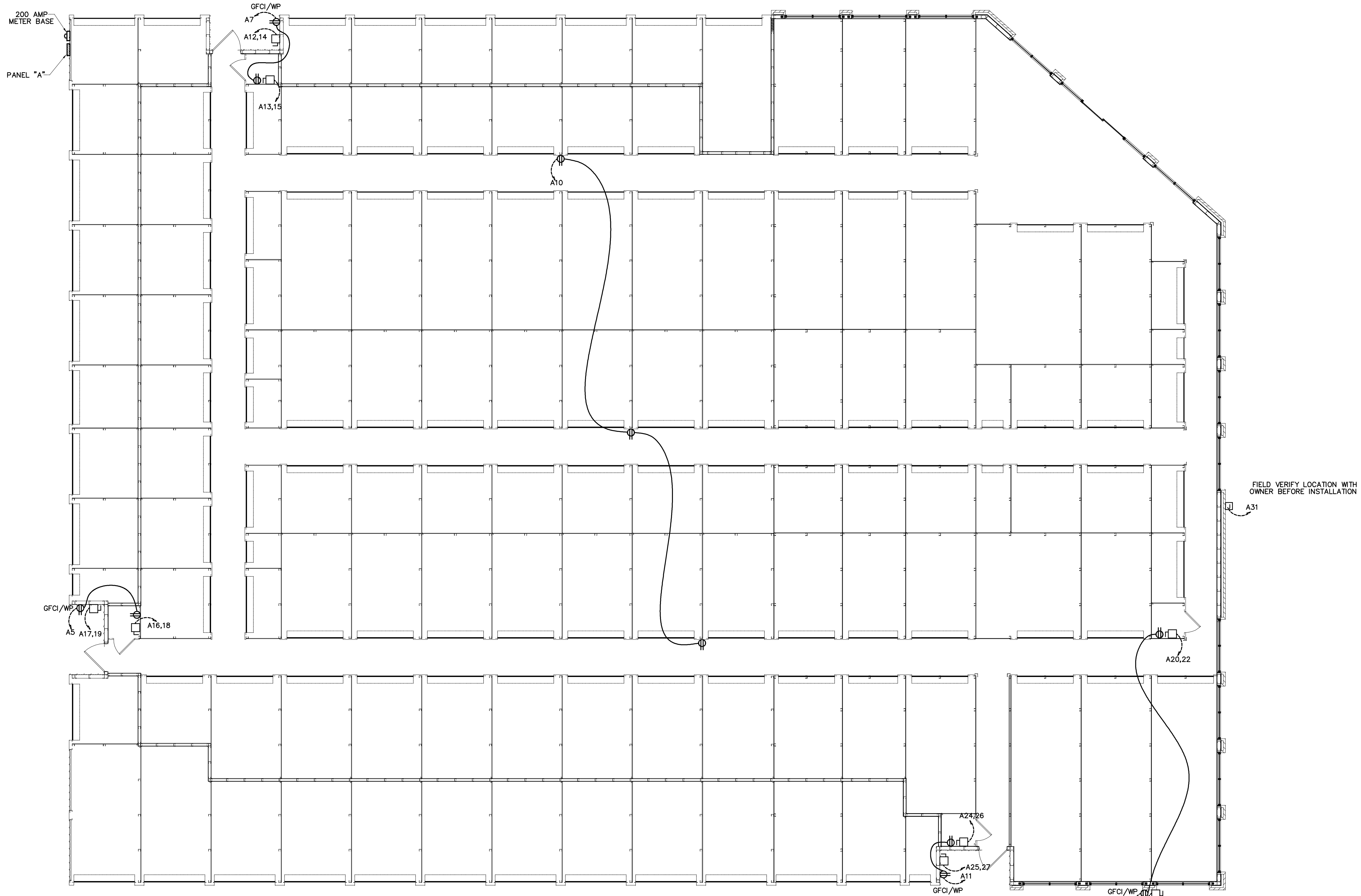
ELECTRICAL POWER PLAN BUILDING "1" SCALE: 1/8" = 1'-0"
