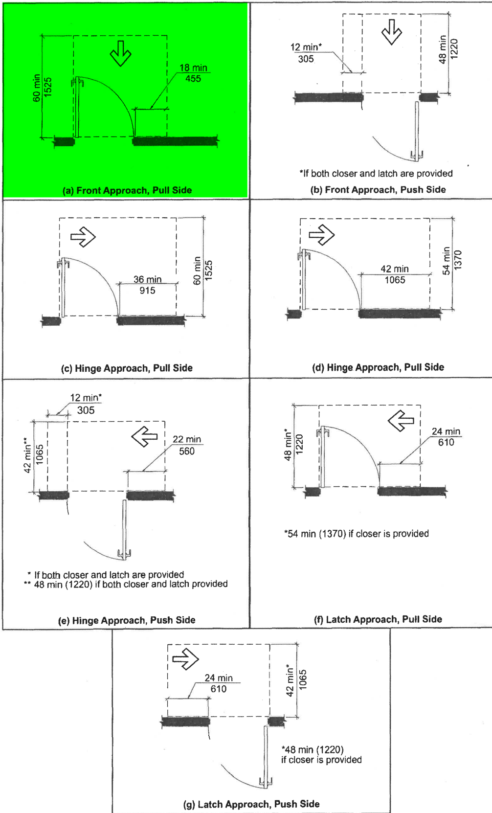
FIG. 404.2.3.2 MANEUVERING CLEARANCE AT MANUAL SWINGING DOORS
