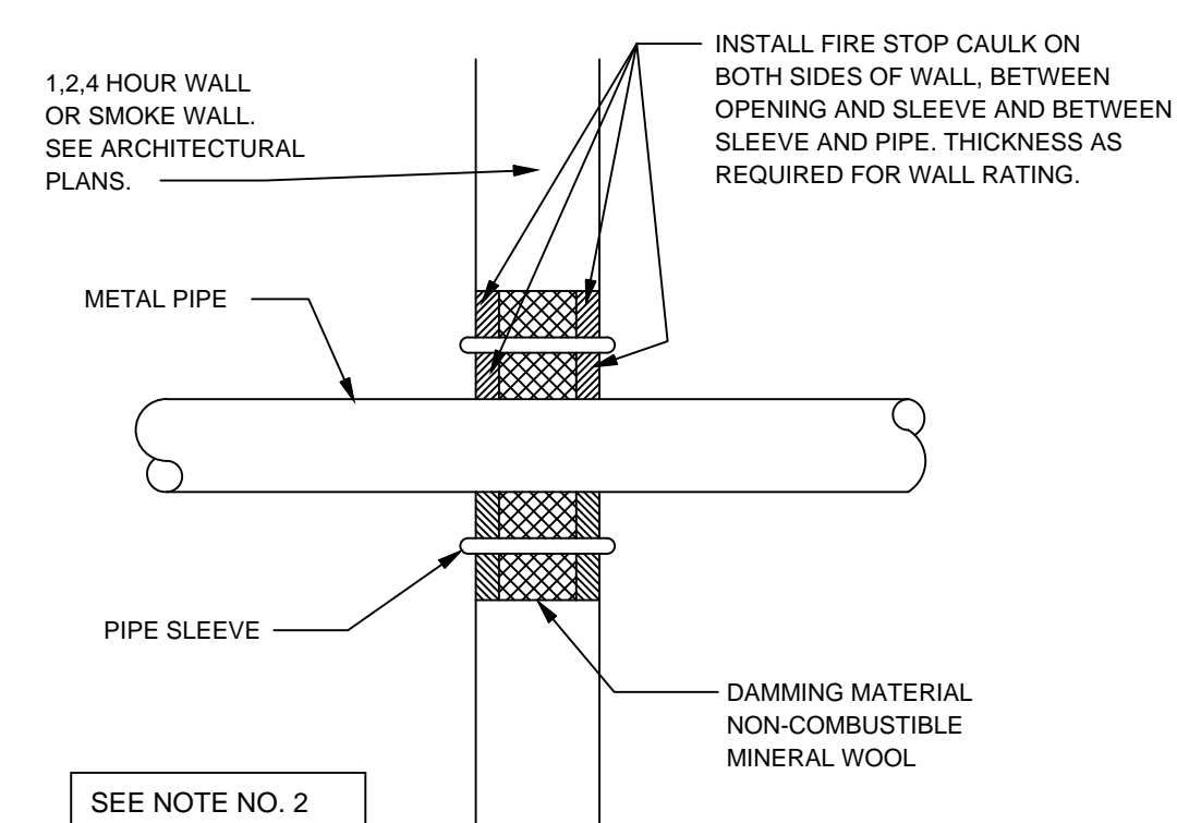
METAL PIPE PENETRATION-WALL (U.L. SYSTEM NO. WL5024)
