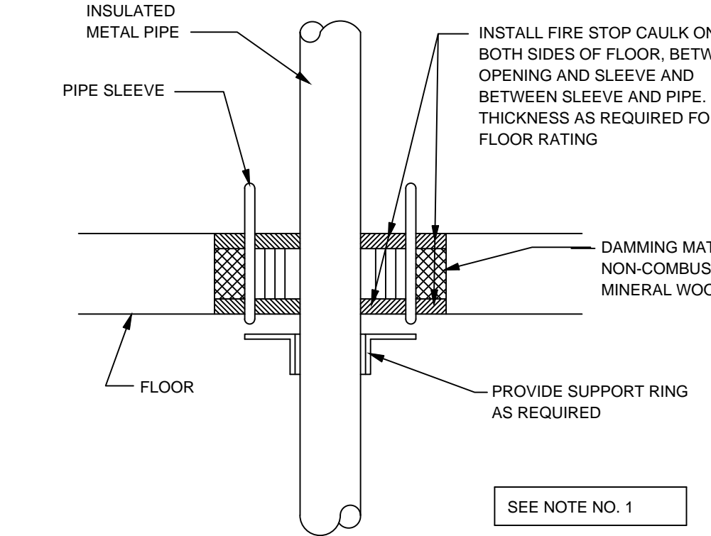
INSULATED METAL PIPE PENETRATION-FLOOR (U.L. SYSTEM NO. CAJ1043) - 1, 2 HR. (U.L. SYSTEM NO. CAJ1044) - 3, 4 HR.
