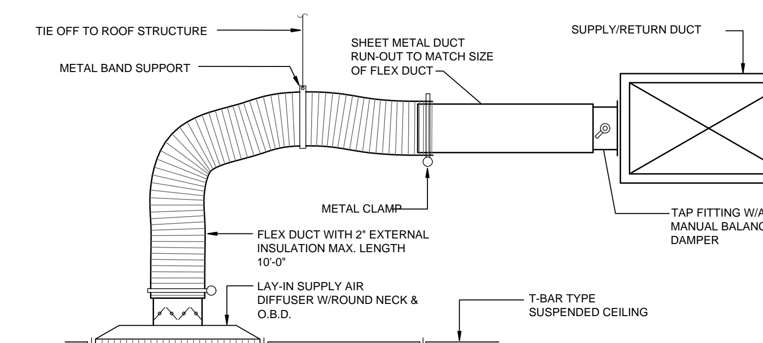
1 AIR DISTRIBUTION DETAIL M07.01 SCALE: NTS
