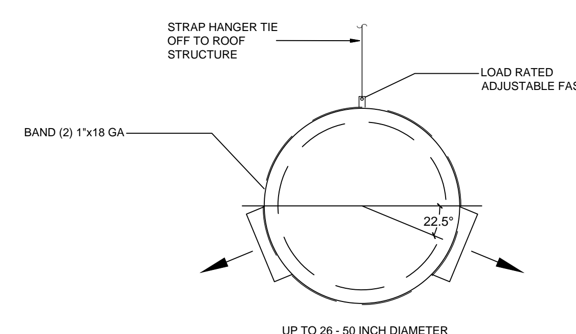
7 SUPPLY REGISTER DETAIL M07.01 SCALE: NTS
