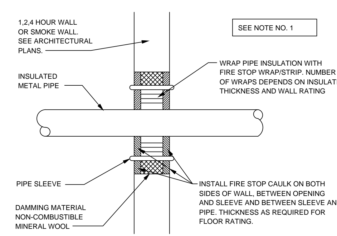
INSULATED METAL PIPE PENETRATION-WALL (U.L. SYSTEM NO. WL5024)
