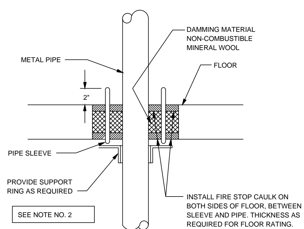
METAL PIPE PENETRATION-FLOOR (U.L. SYSTEM NO. CAJ1043) - 1, 2 HR. (U.L. SYSTEM NO. CAJ1044) - 3, 4 HR.
