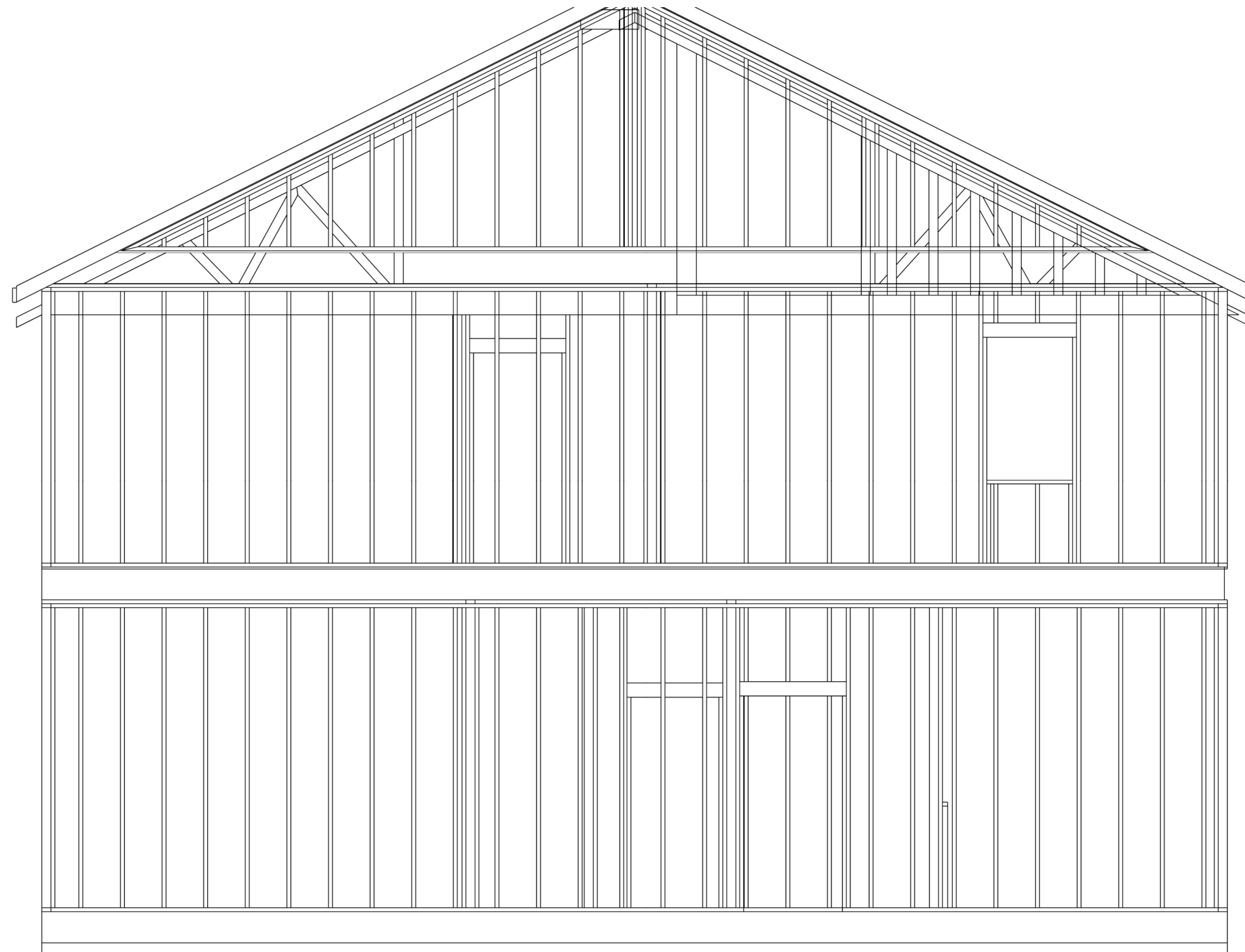
Cross Section 2
