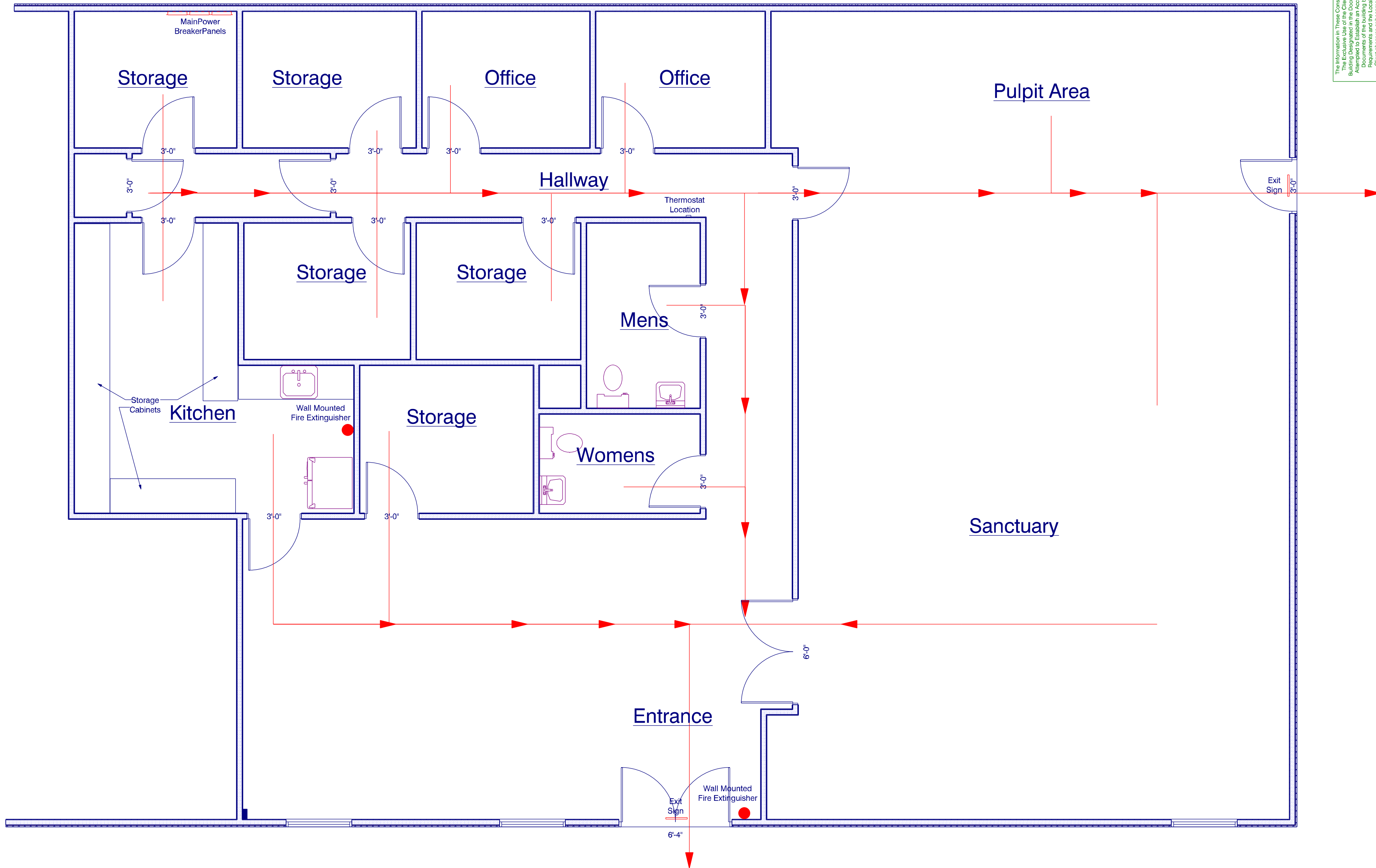
Existing _ New Layout Fire Safety Floorplan Scale: 1/4" = 1' 0"
