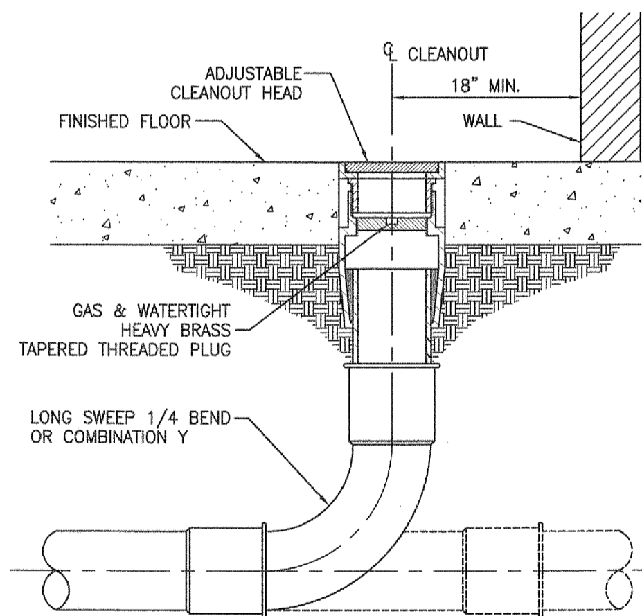
DETAIL NO. 4 FLOOR CLEANOUT WITH SWEEP BEND OR COMBINATION Y SCALE: NTS
