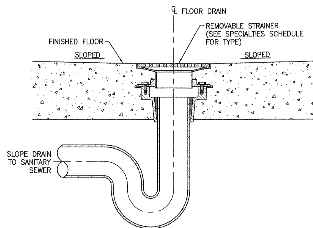
DETAIL NO. 5 FLOOR DRAIN SCALE: NTS
