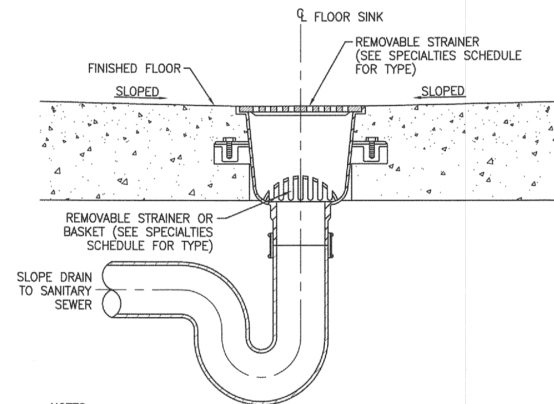
DETAIL NO. 6 FLOOR SINK WITH TRAP PRIMER SCALE: NTS
