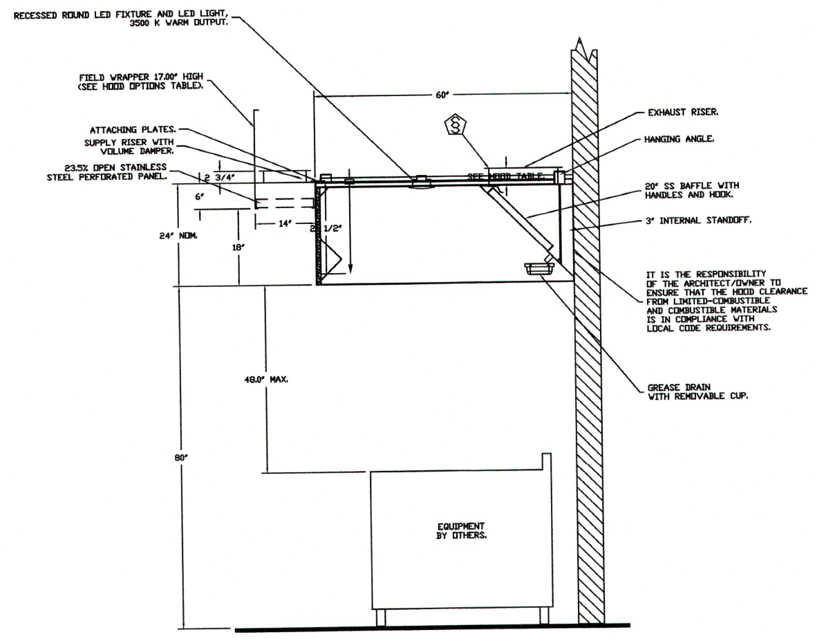
SECTION VIEW - MODEL 6024ND-2-PSP-F HOOD - #2
