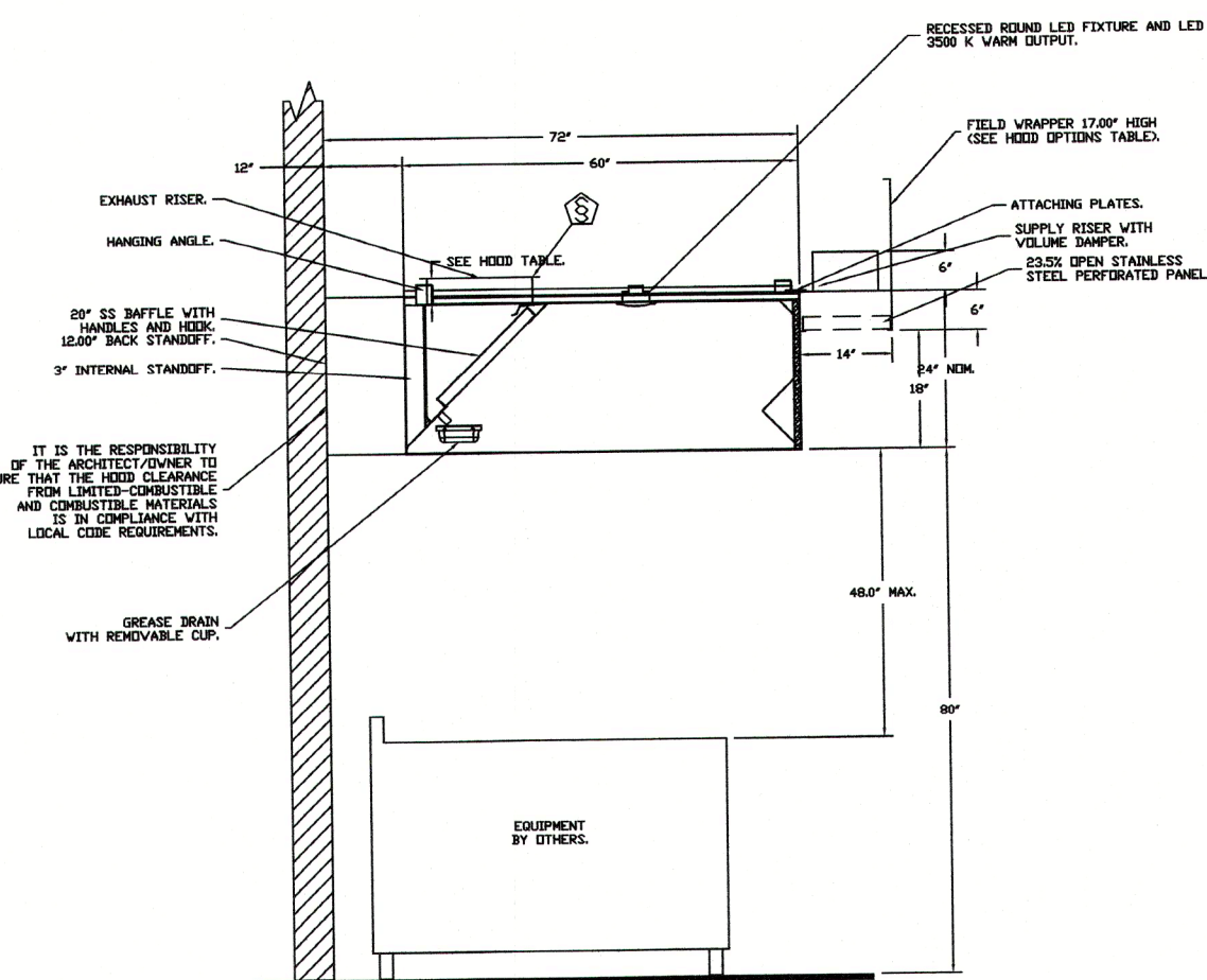
SECTION VIEW - MODEL 6024ND-2-PSP-F HOOD - #1
