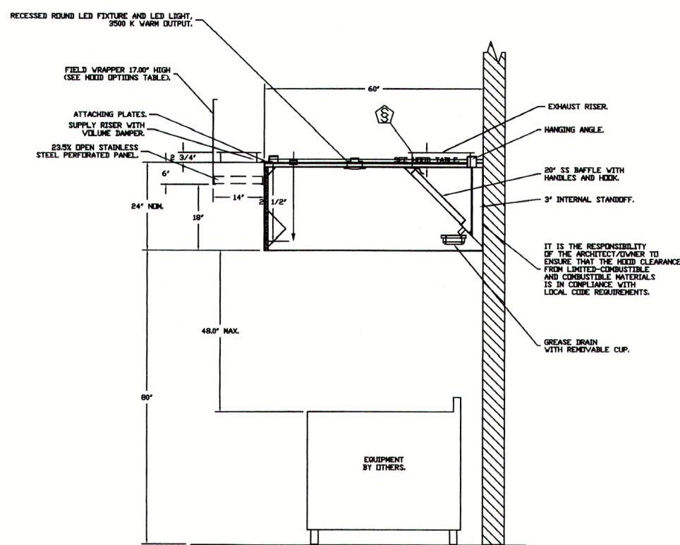
SECTION VIEW - MODEL #024ND-2-PSP-F HOOD - #2
