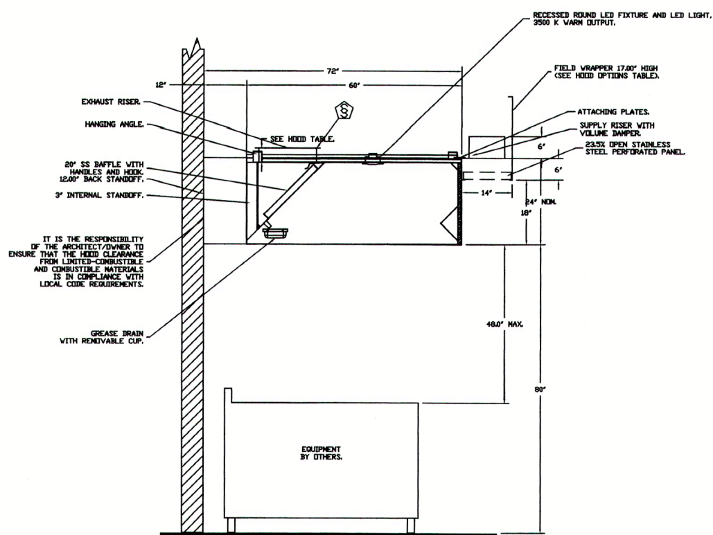
SECTION VIEW - MODEL #024ND-2-PSP-F HOOD - #1
