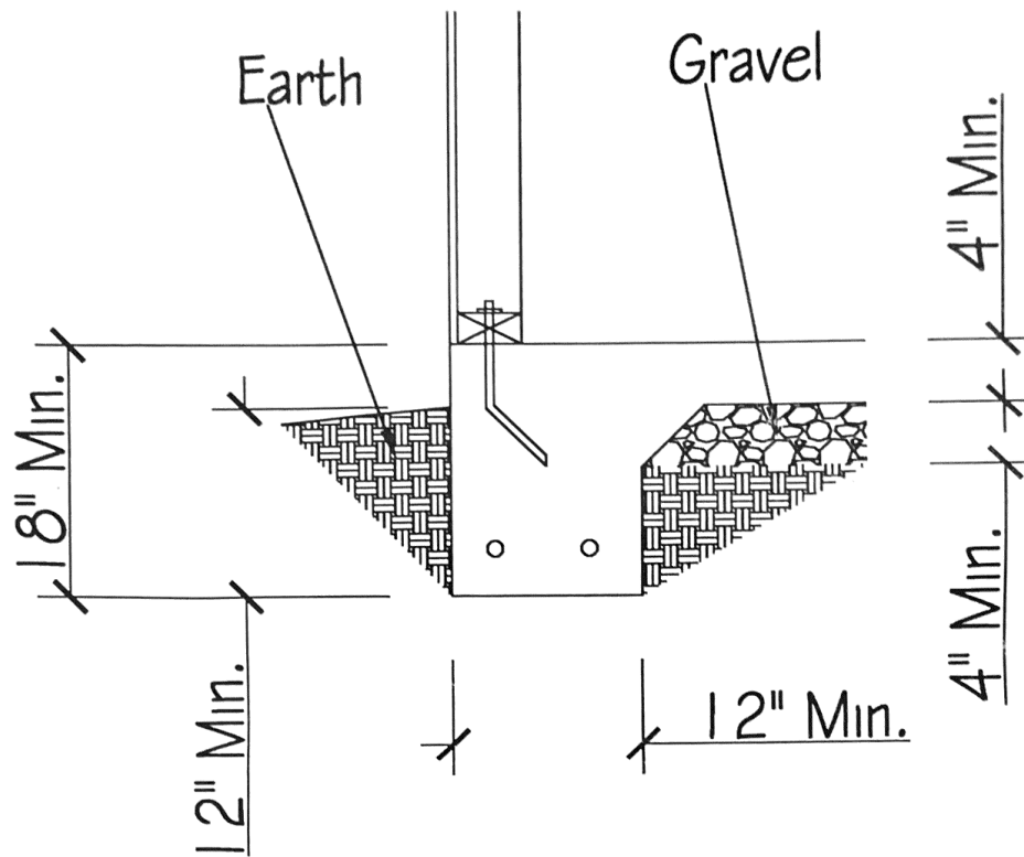
Monolithic Detail
