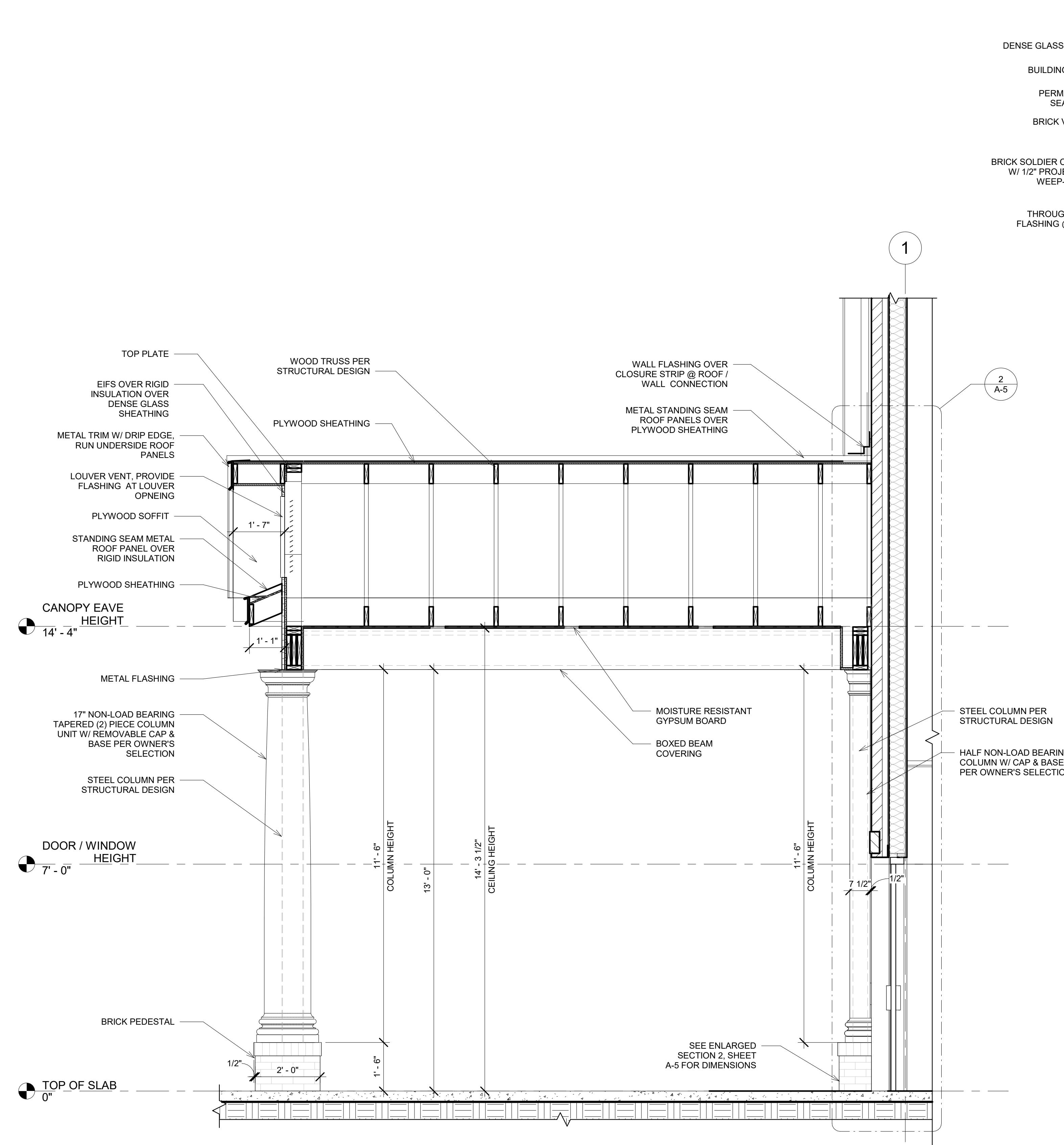
1 SECTION @ FRONT PORTICO 1/2" = 1'-0"
