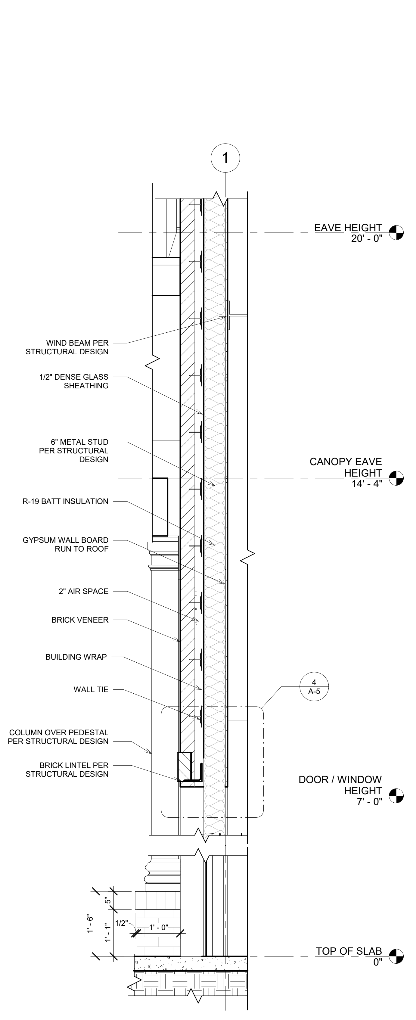
2 ENLARGED SECTION @ GRID LINE 1 3/4" = 1'-0"
