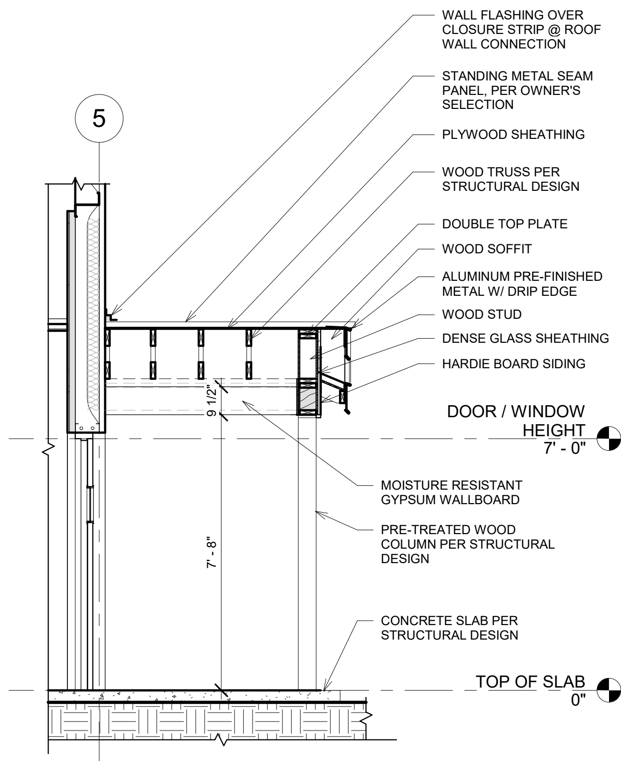
5 SECTION @ REAR CANOPY 3/8" = 1'-0"
