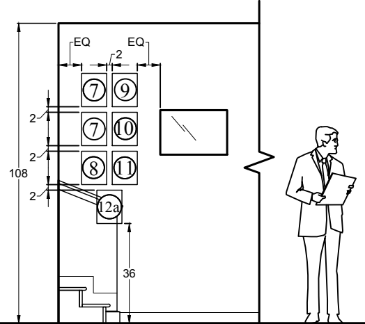
D Gallery Elevation
